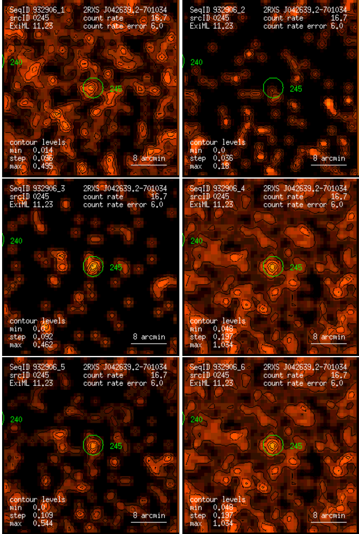
Figure 245: RASS 932906: detection 0245: band rate images, Gaussian filter: (1) PSPC channels 11 – 41, (2) 52 – 90, (3) 91 – 201, (4) 11 – 235, (5) 52 – 201, (6) 11 – 201. Broad band rates in counts/ks. Band rate contour levels in counts/ks/arcmin 2 .
