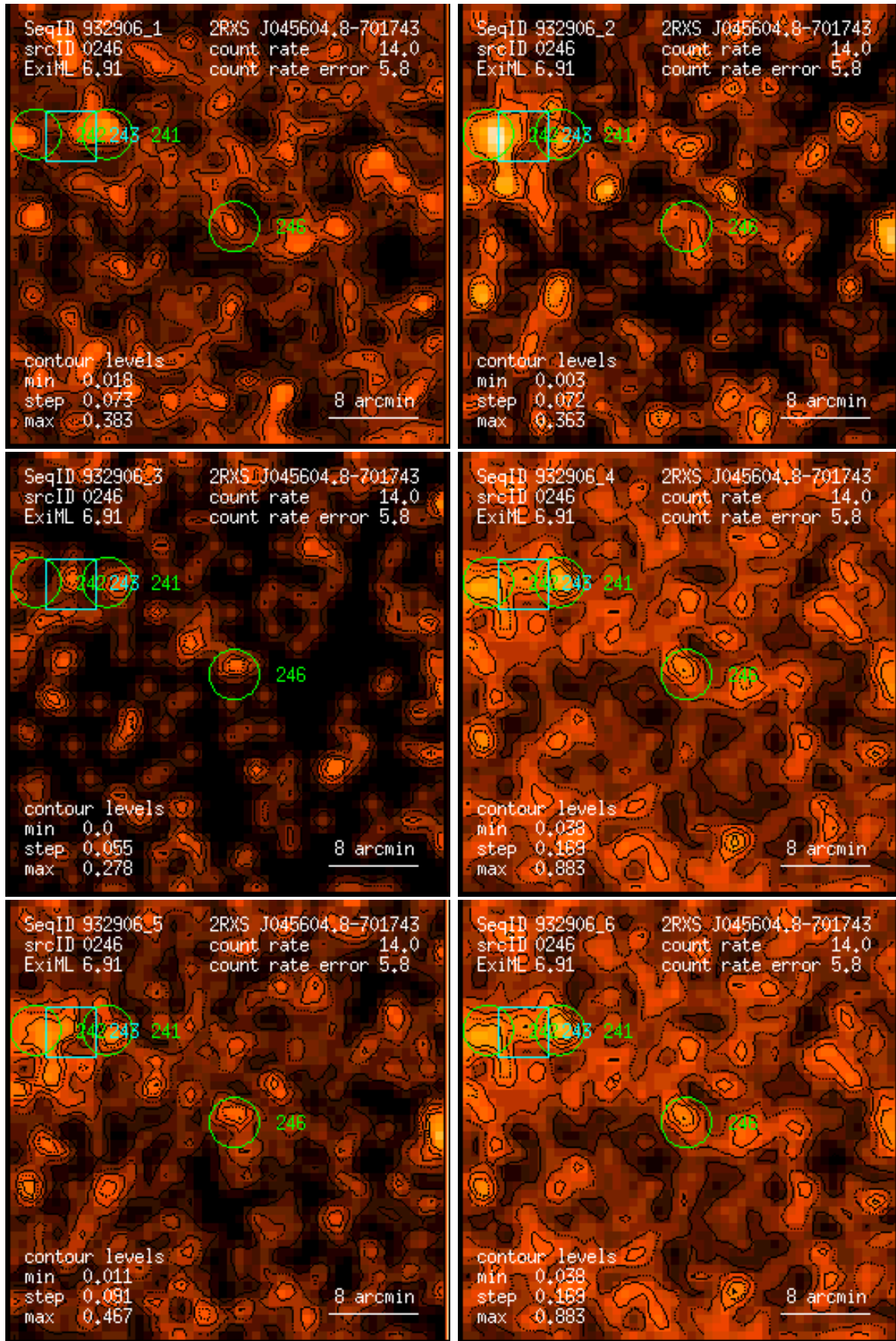
Figure 246: RASS 932906: detection 0246: band rate images, Gaussian filter: (1) PSPC channels 11 – 41, (2) 52 – 90, (3) 91 – 201, (4) 11 – 235, (5) 52 – 201, (6) 11 – 201. Broad band rates in counts/ks. Band rate contour levels in counts/ks/arcmin 2 .
