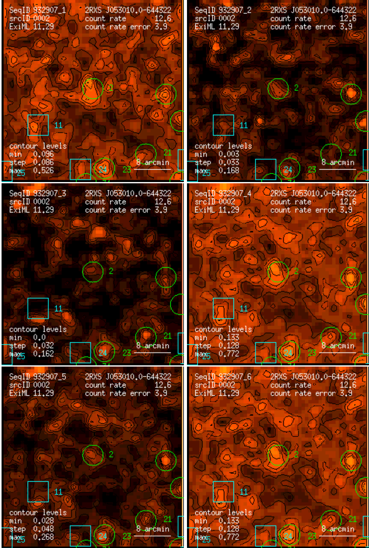
Figure 2: RASS 932907: detection 0002: band rate images, Gaussian filter: (1) PSPC channels 11 – 41, (2) 52 – 90, (3) 91 – 201, (4) 11 – 235, (5) 52 – 201, (6) 11 – 201. Broad band rates in counts/ks. Band rate contour levels in counts/ks/arcmin 2 .
