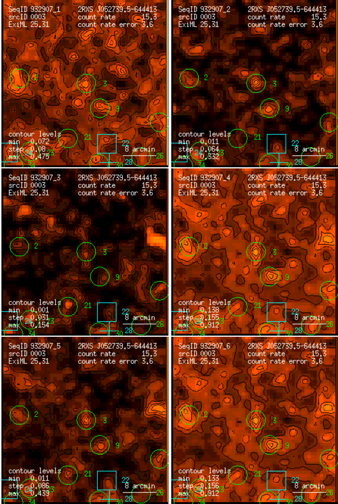
Figure 3: RASS 932907: detection 0003: band rate images, Gaussian filter: (1) PSPC channels 11 – 41, (2) 52 – 90, (3) 91 – 201, (4) 11 – 235, (5) 52 – 201, (6) 11 – 201. Broad band rates in counts/ks. Band rate contour levels in counts/ks/arcmin 2 .
