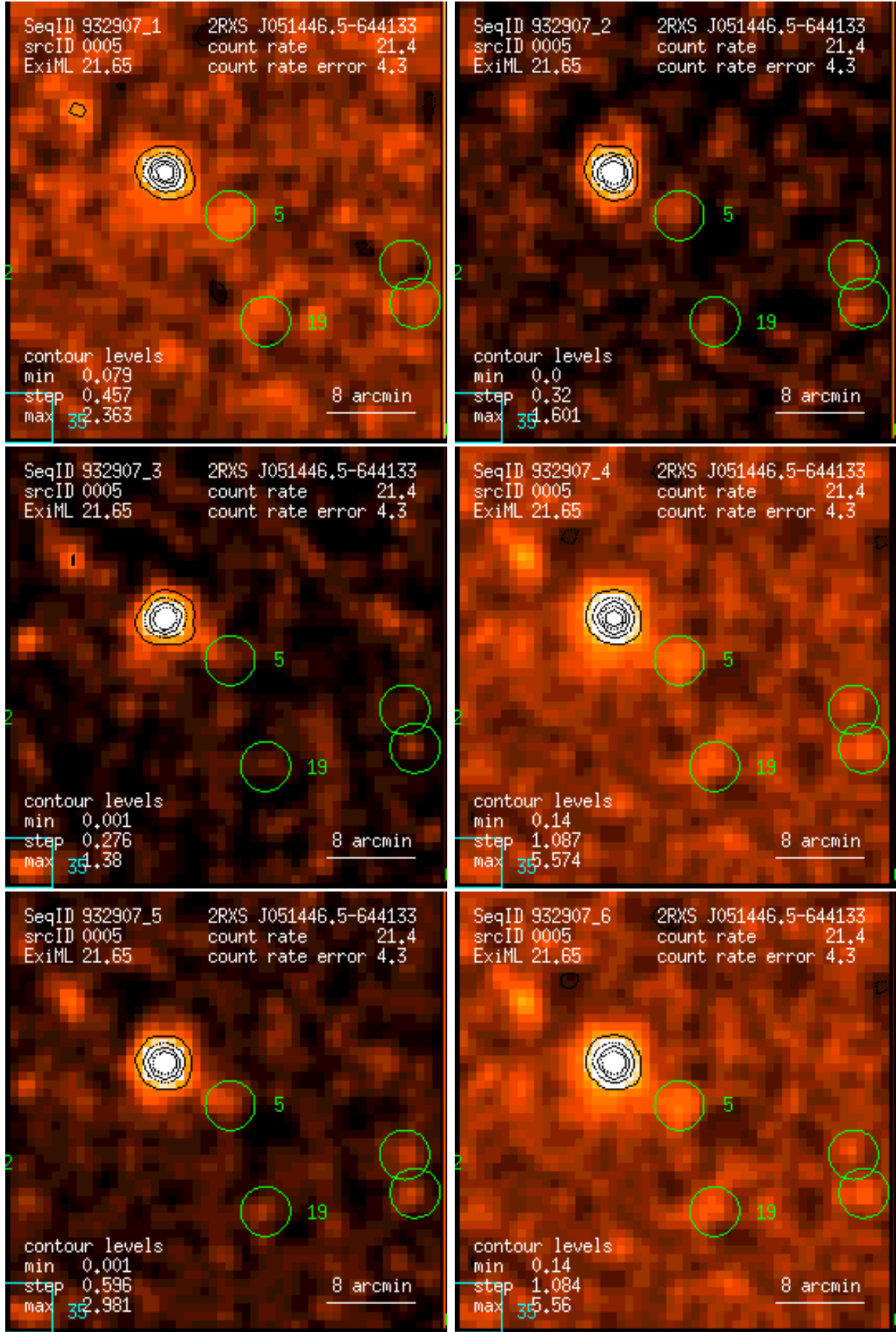
Figure 5: RASS 932907: detection 0005: band rate images, Gaussian filter: (1) PSPC channels 11 – 41, (2) 52 – 90, (3) 91 – 201, (4) 11 – 235, (5) 52 – 201, (6) 11 – 201. Broad band rates in counts/ks. Band rate contour levels in counts/ks/arcmin 2 .
