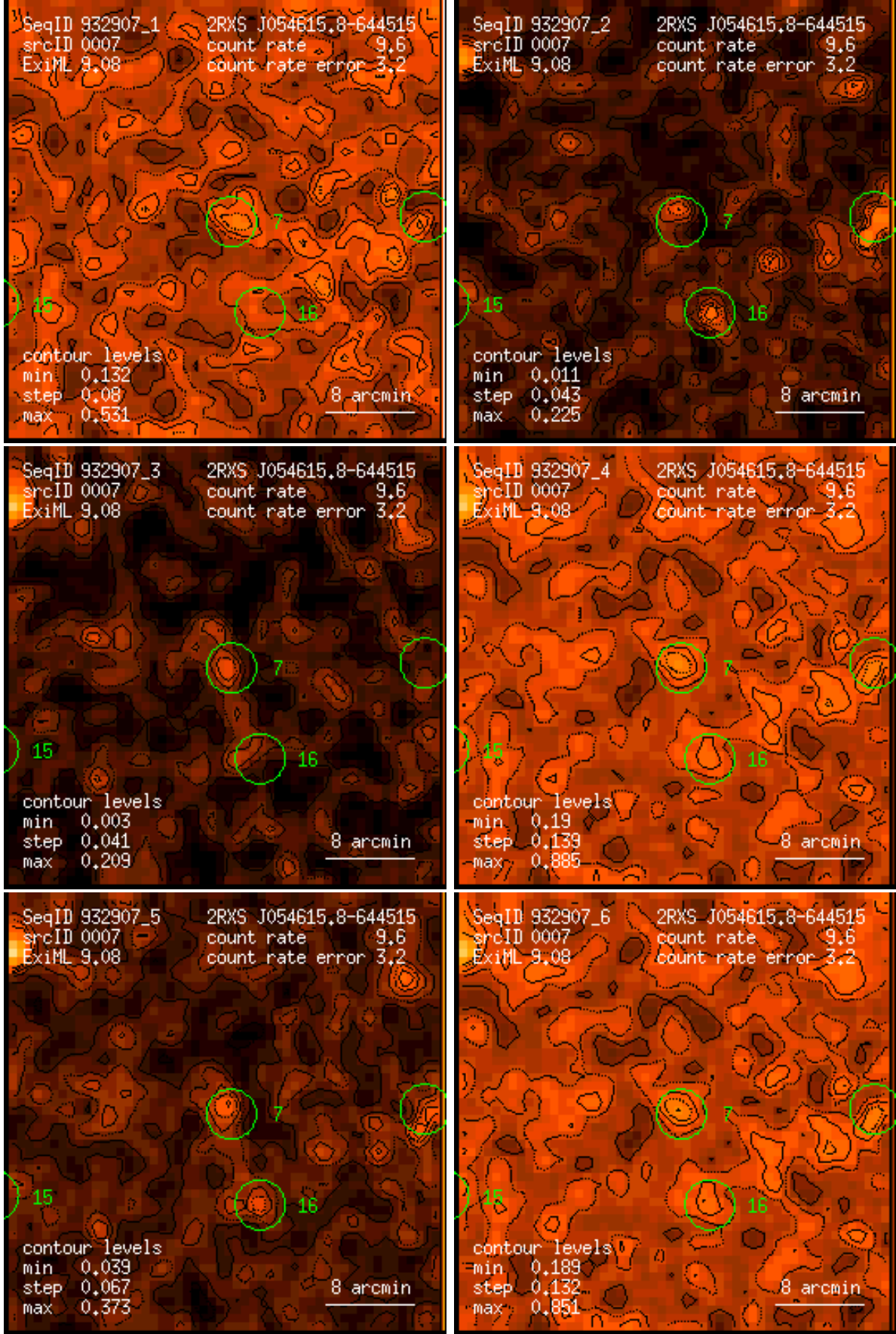
Figure 7: RASS 932907: detection 0007: band rate images, Gaussian filter: (1) PSPC channels 11 – 41, (2) 52 – 90, (3) 91 – 201, (4) 11 – 235, (5) 52 – 201, (6) 11 – 201. Broad band rates in counts/ks. Band rate contour levels in counts/ks/arcmin 2 .
