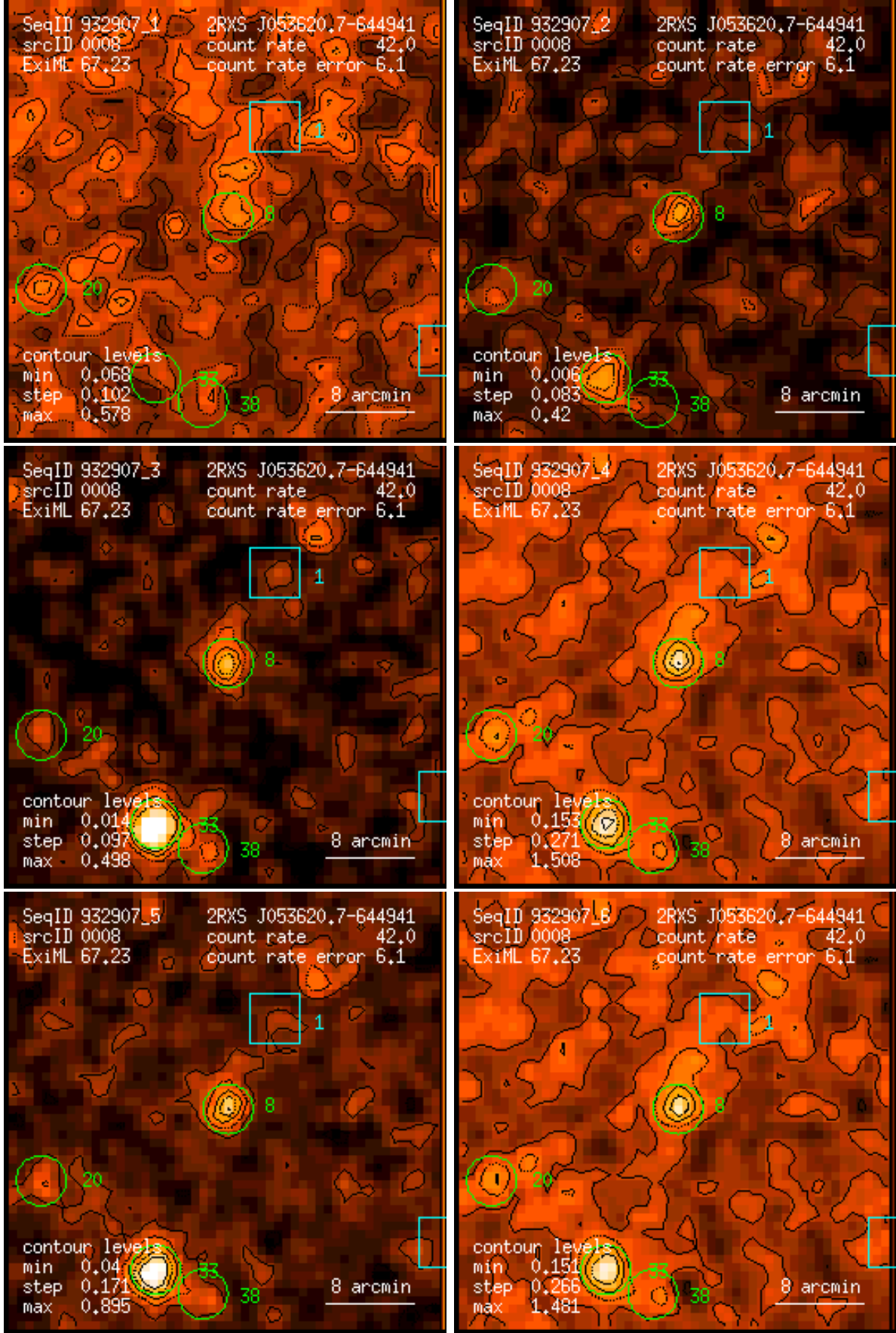
Figure 8: RASS 932907: detection 0008: band rate images, Gaussian filter: (1) PSPC channels 11 – 41, (2) 52 – 90, (3) 91 – 201, (4) 11 – 235, (5) 52 – 201, (6) 11 – 201. Broad band rates in counts/ks. Band rate contour levels in counts/ks/arcmin 2 .
