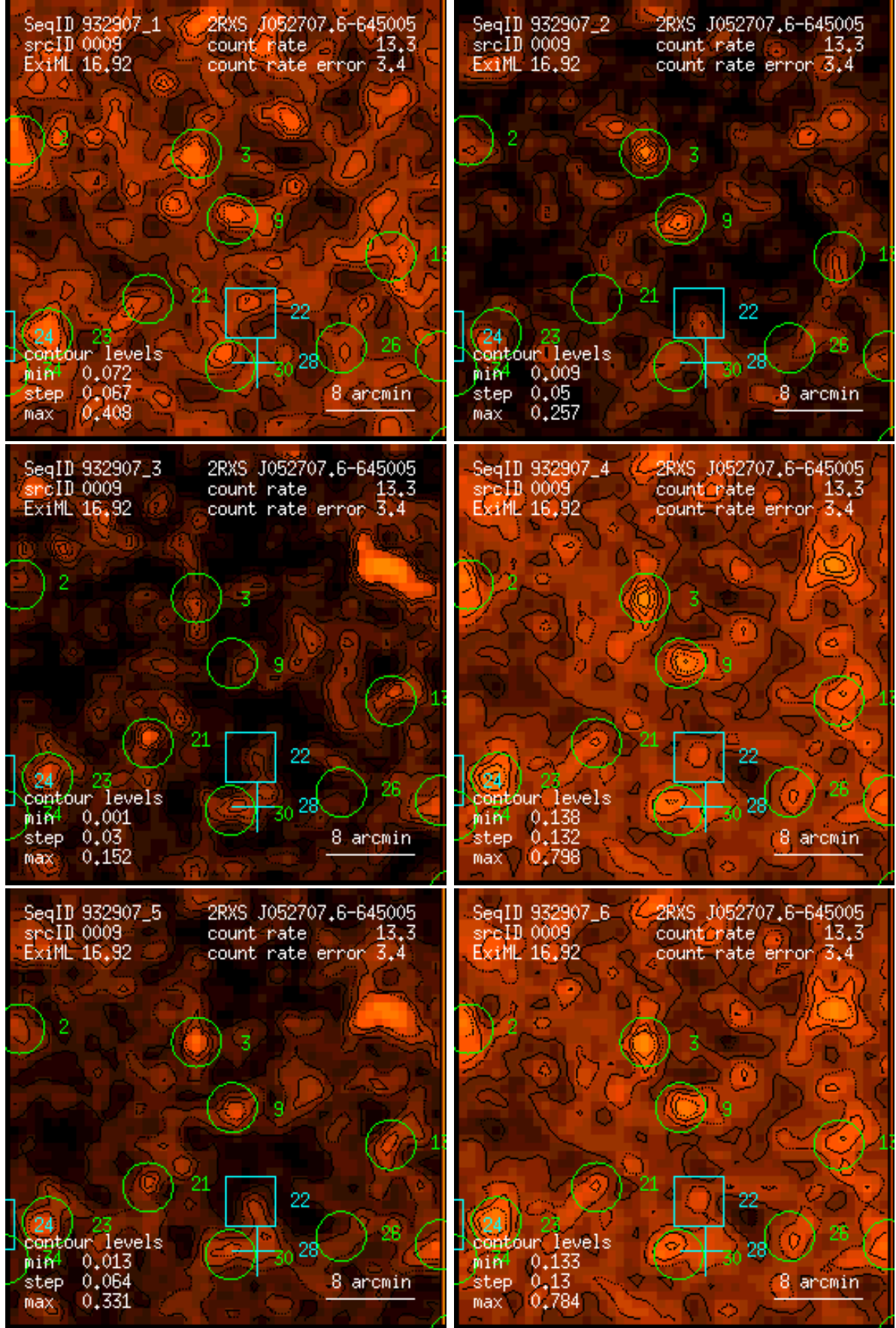
Figure 9: RASS 932907: detection 0009: band rate images, Gaussian filter: (1) PSPC channels 11 – 41, (2) 52 – 90, (3) 91 – 201, (4) 11 – 235, (5) 52 – 201, (6) 11 – 201. Broad band rates in counts/ks. Band rate contour levels in counts/ks/arcmin 2 .
