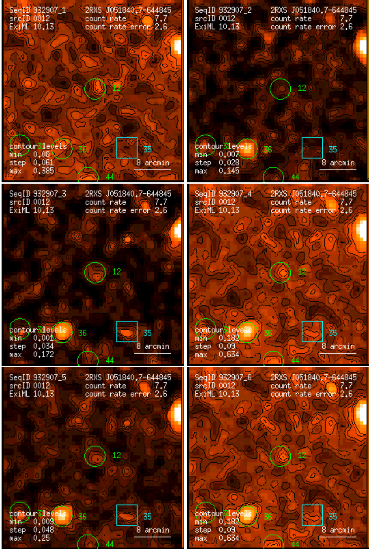
Figure 12: RASS 932907: detection 0012: band rate images, Gaussian filter: (1) PSPC channels 11 – 41, (2) 52 – 90, (3) 91 – 201, (4) 11 – 235, (5) 52 – 201, (6) 11 – 201. Broad band rates in counts/ks. Band rate contour levels in counts/ks/arcmin 2 .
