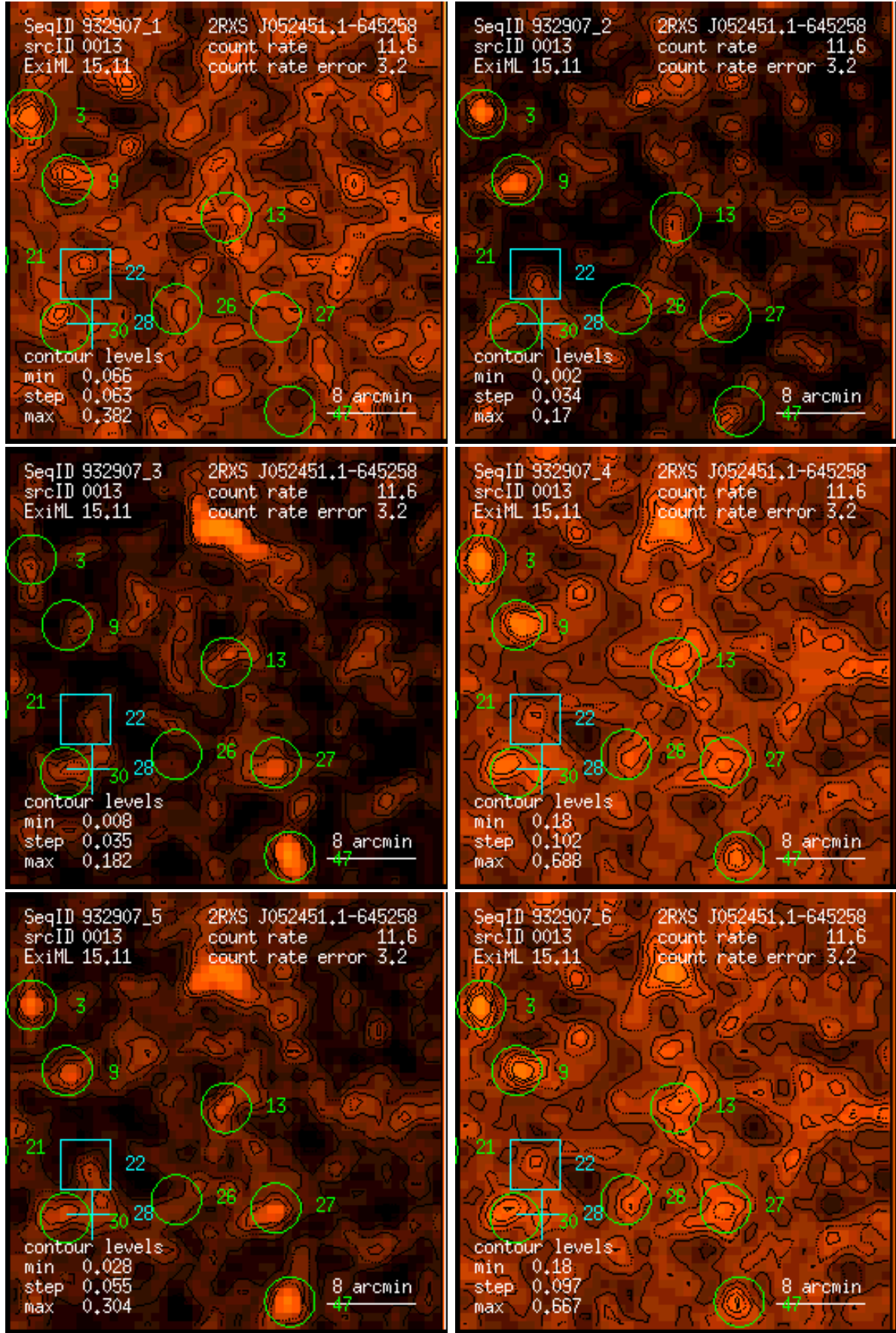
Figure 13: RASS 932907: detection 0013: band rate images, Gaussian filter: (1) PSPC channels 11 – 41, (2) 52 – 90, (3) 91 – 201, (4) 11 – 235, (5) 52 – 201, (6) 11 – 201. Broad band rates in counts/ks. Band rate contour levels in counts/ks/arcmin 2 .
