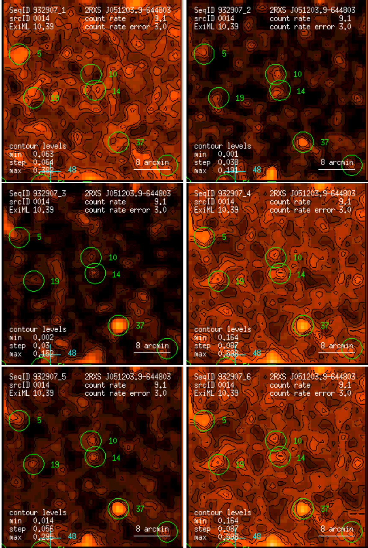
Figure 14: RASS 932907: detection 0014: band rate images, Gaussian filter: (1) PSPC channels 11 – 41, (2) 52 – 90, (3) 91 – 201, (4) 11 – 235, (5) 52 – 201, (6) 11 – 201. Broad band rates in counts/ks. Band rate contour levels in counts/ks/arcmin 2 .
