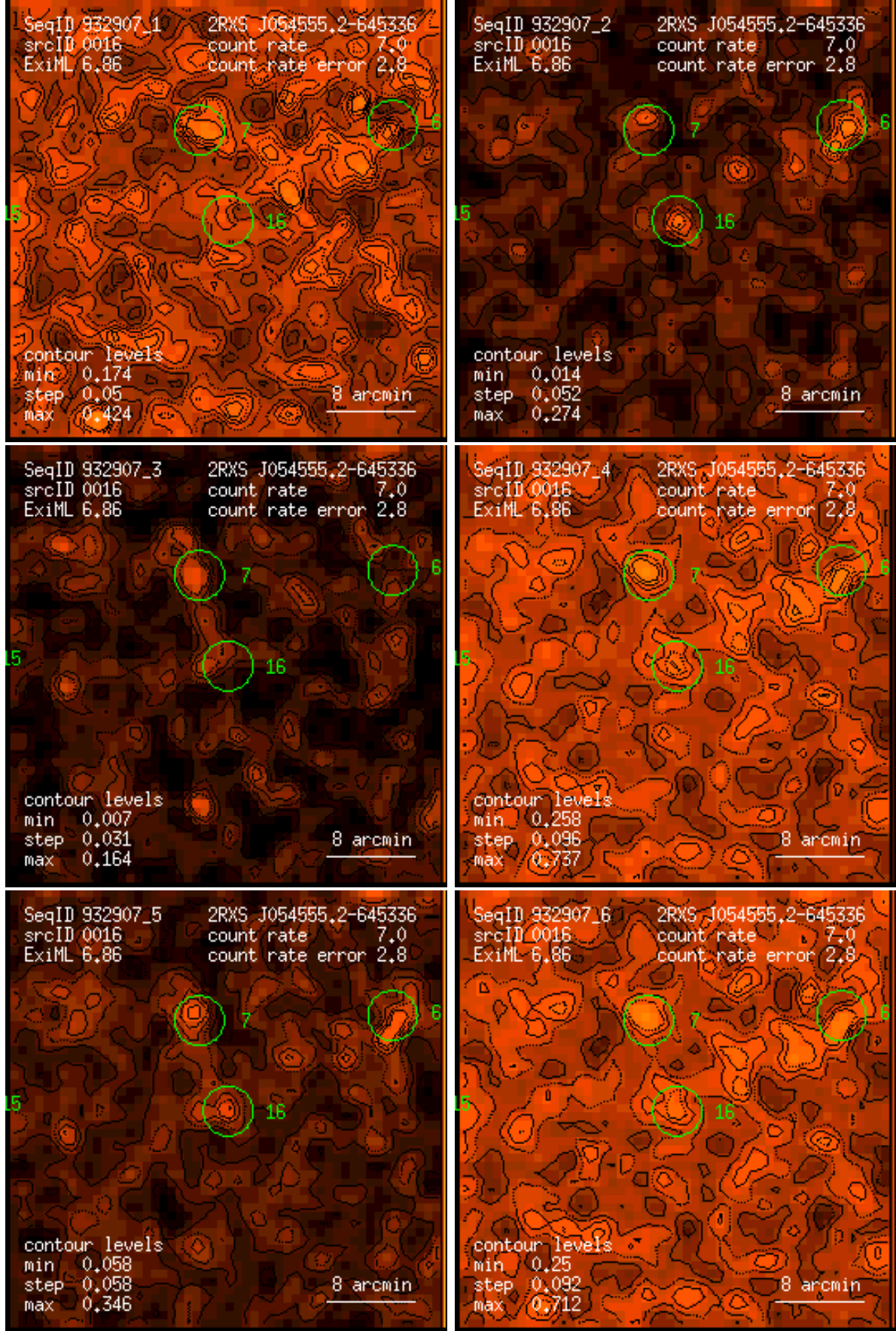
Figure 16: RASS 932907: detection 0016: band rate images, Gaussian filter: (1) PSPC channels 11 – 41, (2) 52 – 90, (3) 91 – 201, (4) 11 – 235, (5) 52 – 201, (6) 11 – 201. Broad band rates in counts/ks. Band rate contour levels in counts/ks/arcmin 2 .
