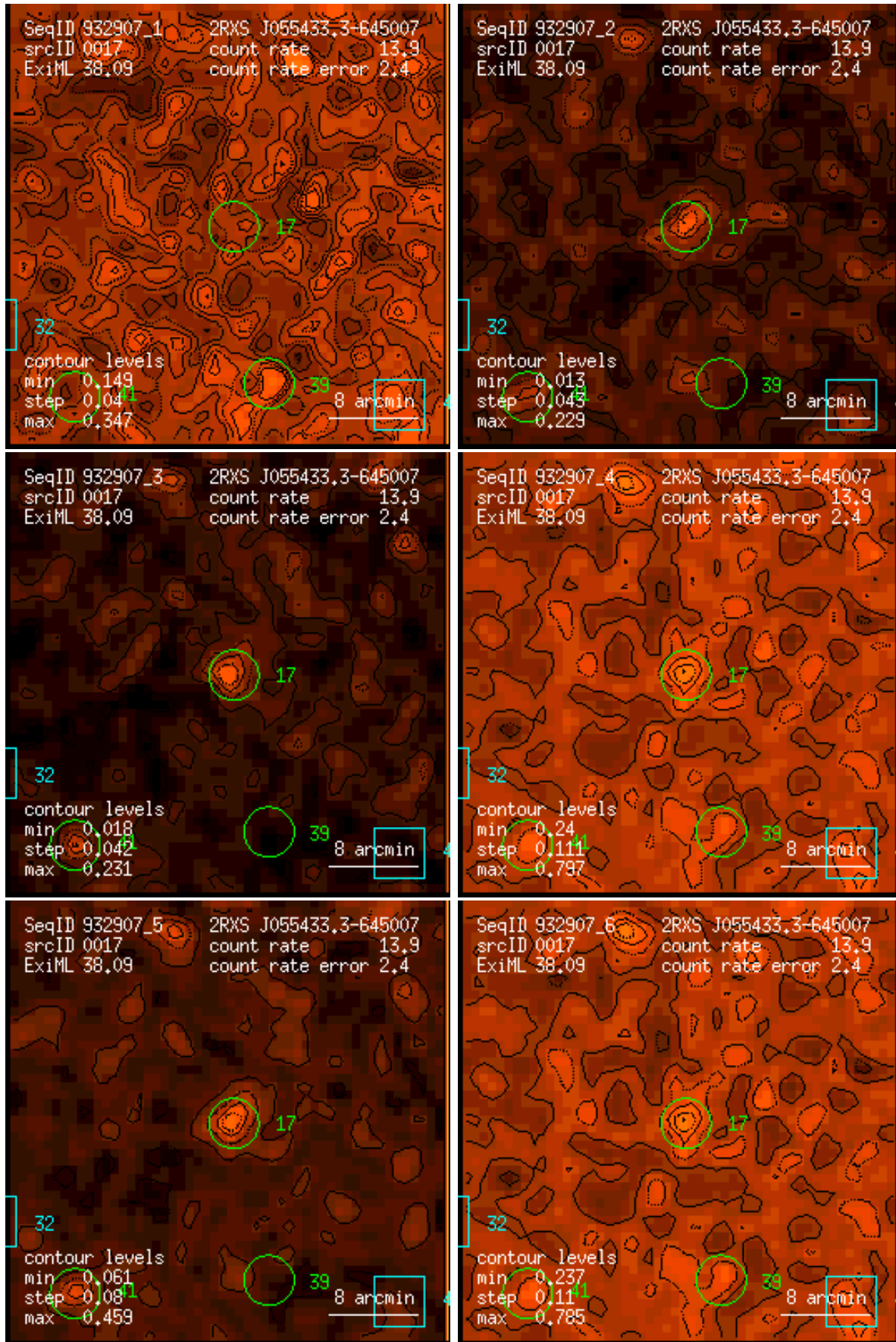
Figure 17: RASS 932907: detection 0017: band rate images, Gaussian filter: (1) PSPC channels 11 – 41, (2) 52 – 90, (3) 91 – 201, (4) 11 – 235, (5) 52 – 201, (6) 11 – 201. Broad band rates in counts/ks. Band rate contour levels in counts/ks/arcmin 2 .
