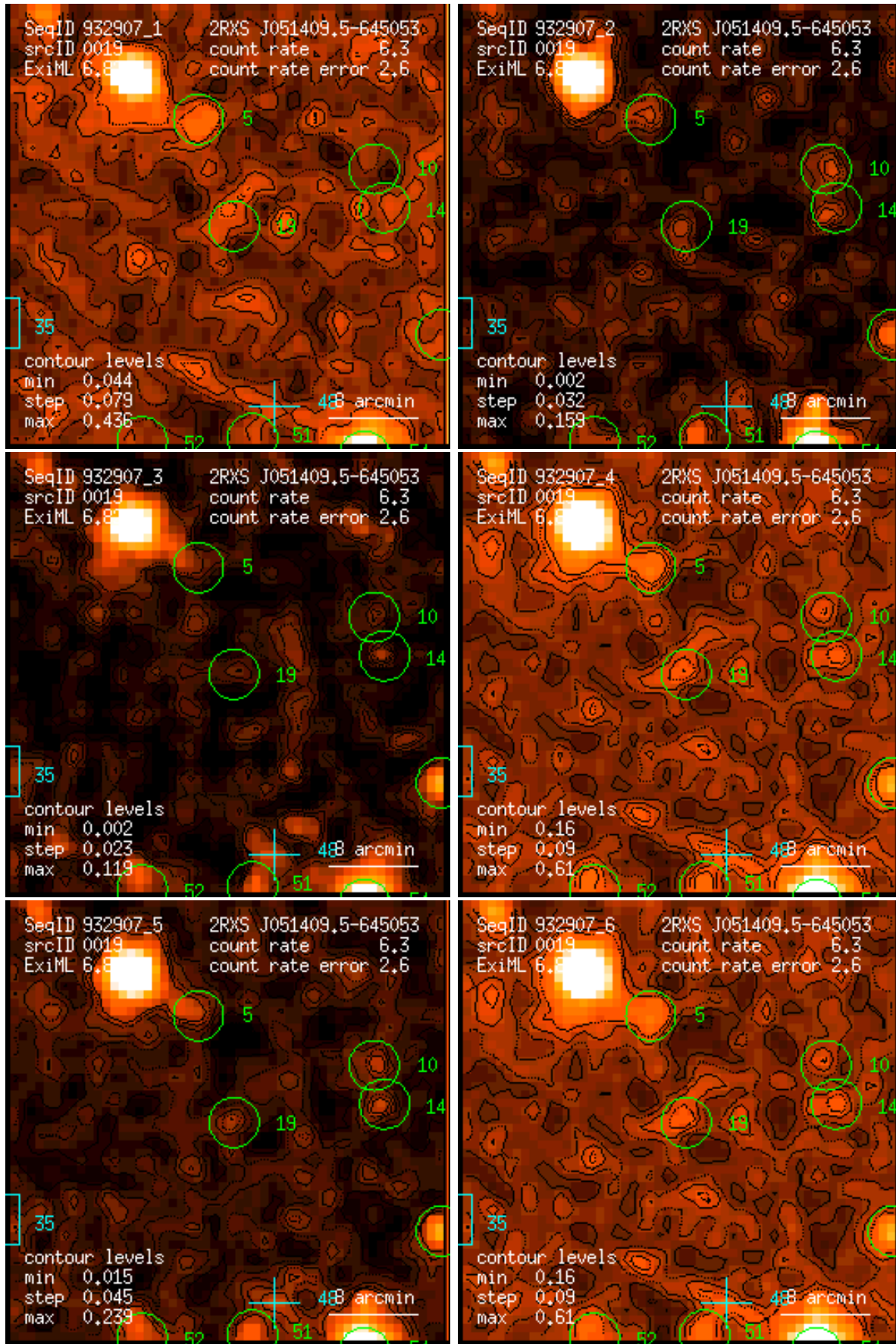
Figure 19: RASS 932907: detection 0019: band rate images, Gaussian filter: (1) PSPC channels 11 – 41, (2) 52 – 90, (3) 91 – 201, (4) 11 – 235, (5) 52 – 201, (6) 11 – 201. Broad band rates in counts/ks. Band rate contour levels in counts/ks/arcmin 2 .
