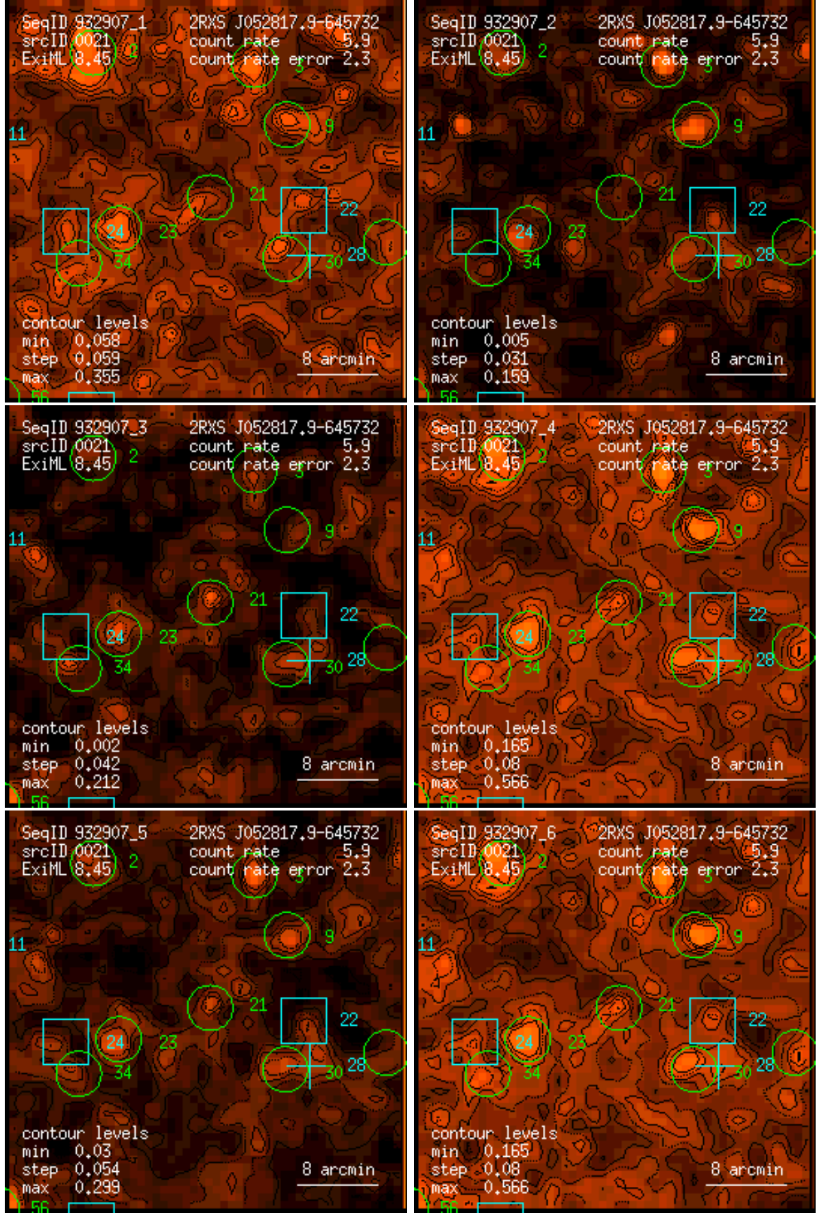
Figure 21: RASS 932907: detection 0021: band rate images, Gaussian filter: (1) PSPC channels 11 – 41, (2) 52 – 90, (3) 91 – 201, (4) 11 – 235, (5) 52 – 201, (6) 11 – 201. Broad band rates in counts/ks. Band rate contour levels in counts/ks/arcmin 2 .
