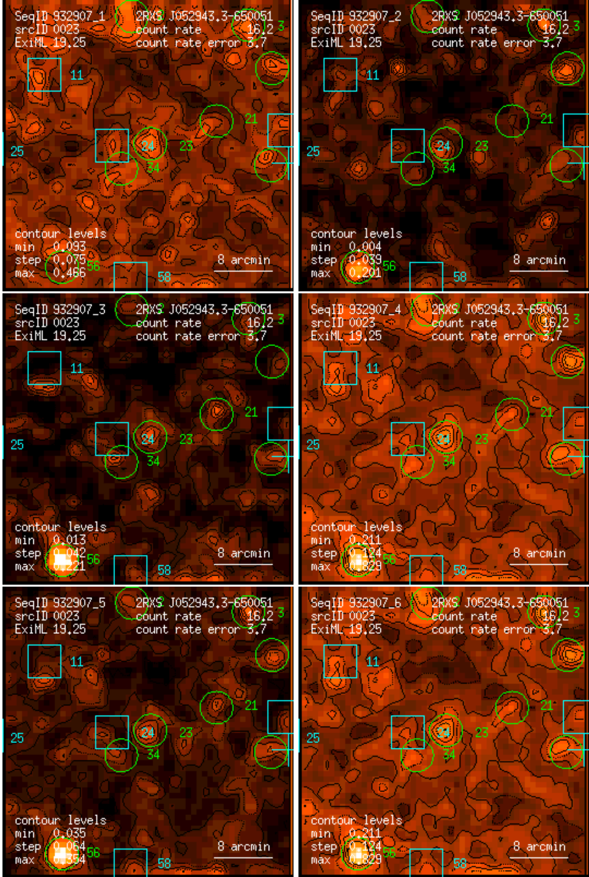
Figure 23: RASS 932907: detection 0023: band rate images, Gaussian filter: (1) PSPC channels 11 – 41, (2) 52 – 90, (3) 91 – 201, (4) 11 – 235, (5) 52 – 201, (6) 11 – 201. Broad band rates in counts/ks. Band rate contour levels in counts/ks/arcmin 2 .
