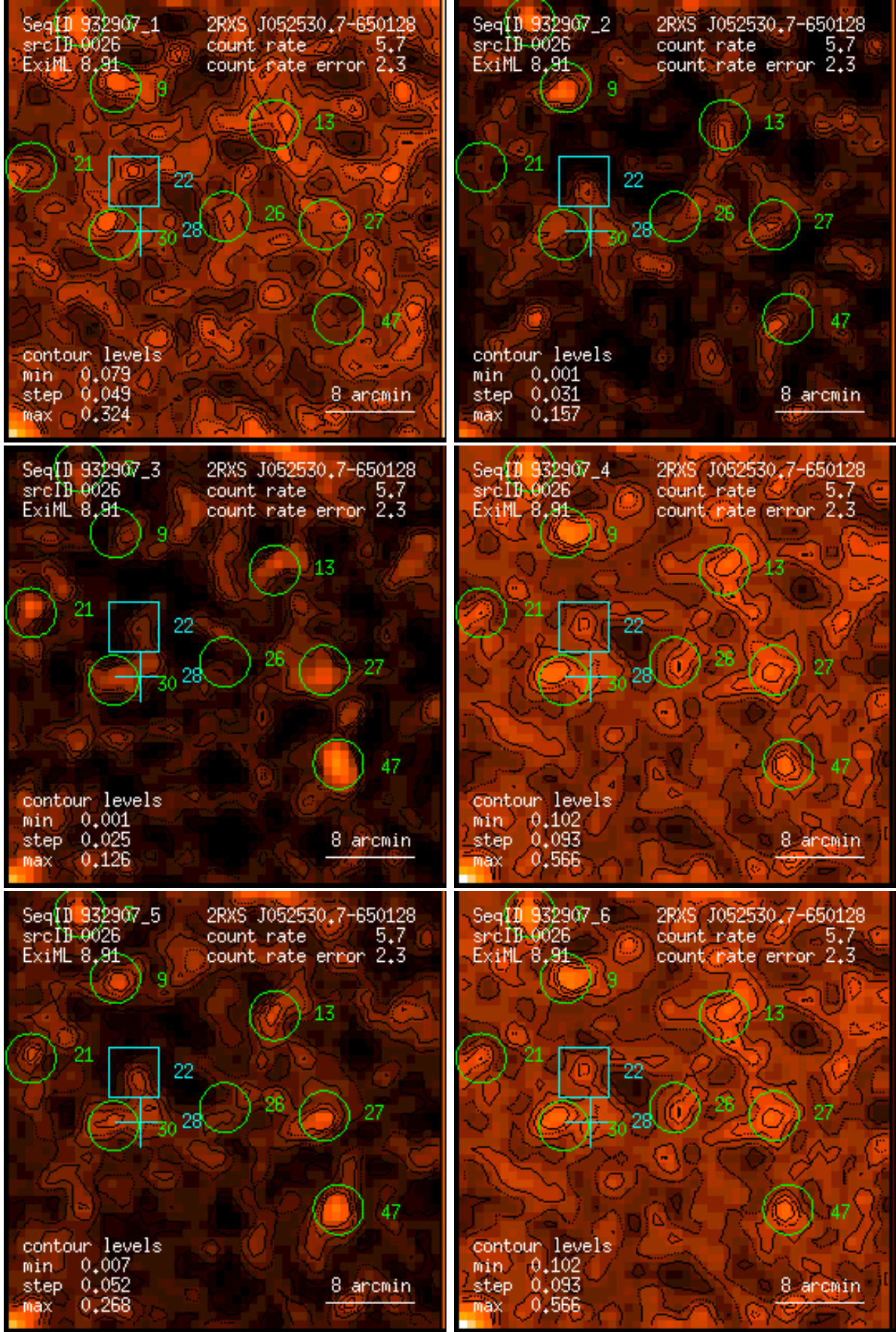
Figure 26: RASS 932907: detection 0026: band rate images, Gaussian filter: (1) PSPC channels 11 – 41, (2) 52 – 90, (3) 91 – 201, (4) 11 – 235, (5) 52 – 201, (6) 11 – 201. Broad band rates in counts/ks. Band rate contour levels in counts/ks/arcmin 2 .
