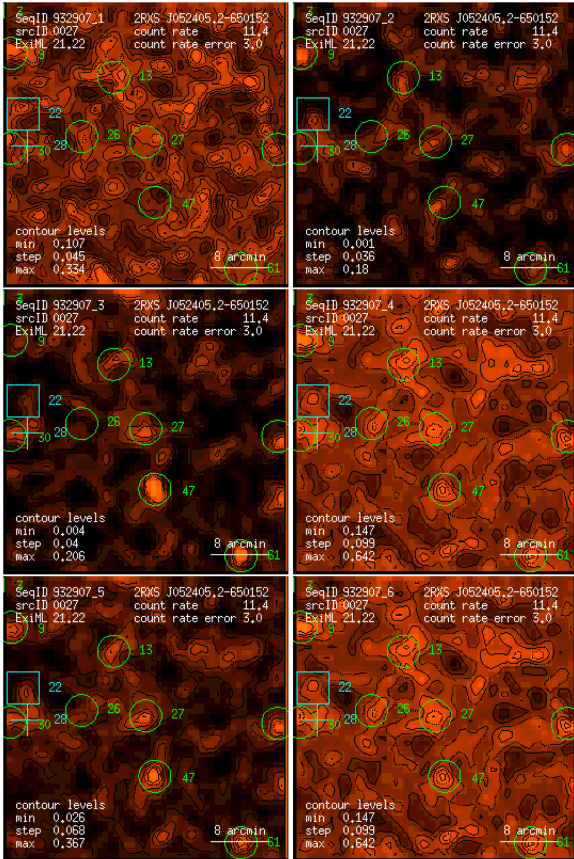
Figure 27: RASS 932907: detection 0027: band rate images, Gaussian filter: (1) PSPC channels 11 – 41, (2) 52 – 90, (3) 91 – 201, (4) 11 – 235, (5) 52 – 201, (6) 11 – 201. Broad band rates in counts/ks. Band rate contour levels in counts/ks/arcmin 2 .
