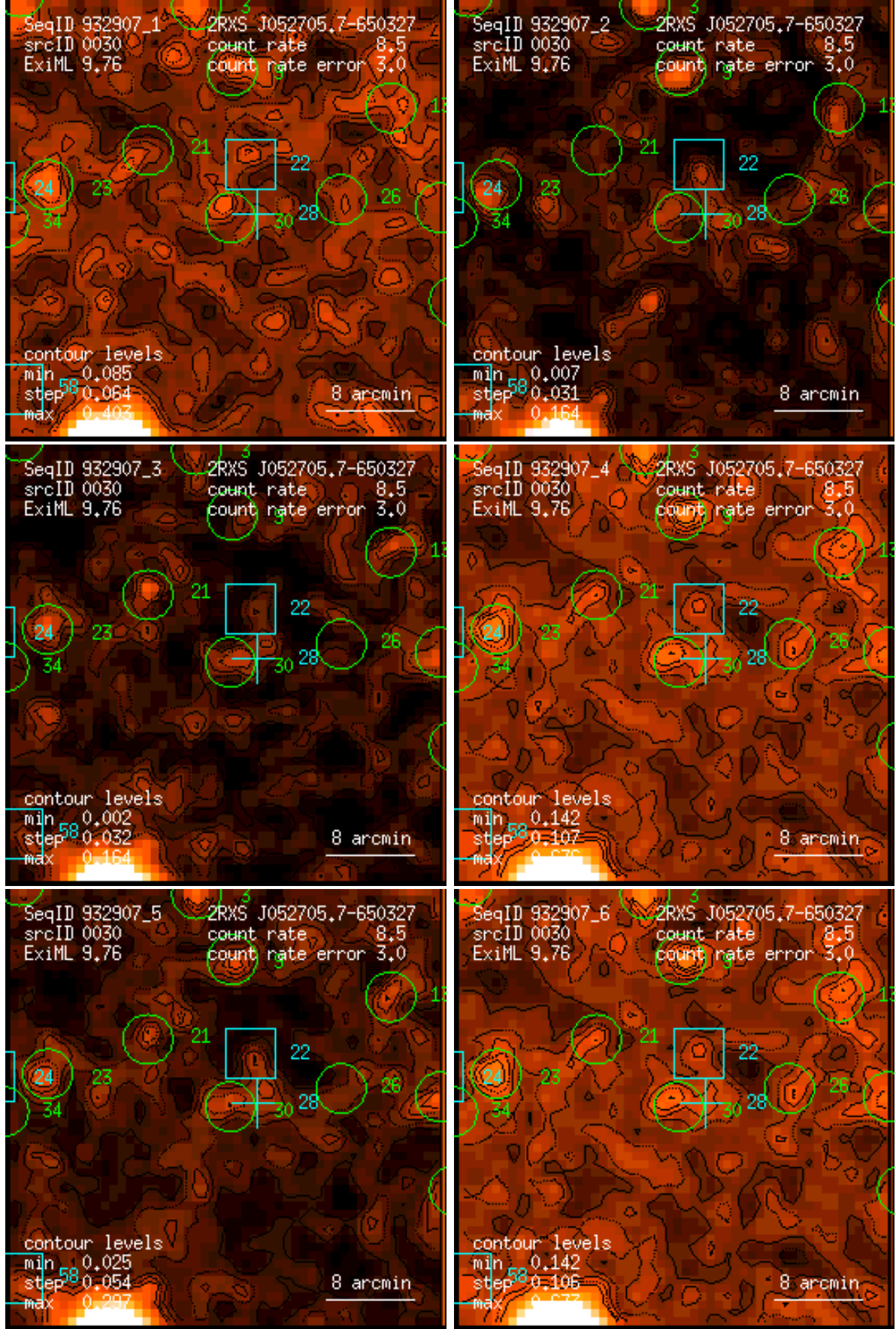
Figure 30: RASS 932907: detection 0030: band rate images, Gaussian filter: (1) PSPC channels 11 – 41, (2) 52 – 90, (3) 91 – 201, (4) 11 – 235, (5) 52 – 201, (6) 11 – 201. Broad band rates in counts/ks. Band rate contour levels in counts/ks/arcmin 2 .
