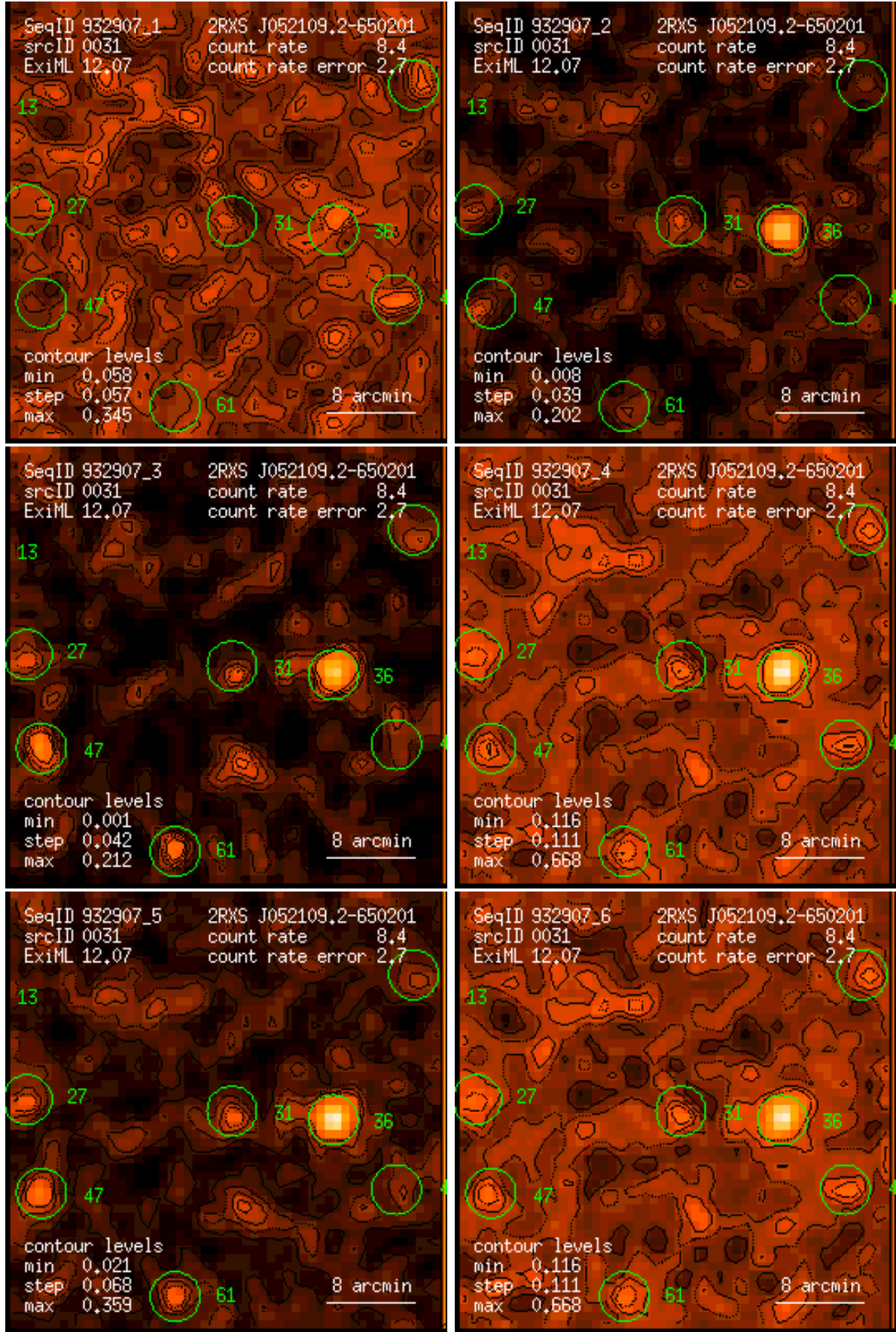
Figure 31: RASS 932907: detection 0031: band rate images, Gaussian filter: (1) PSPC channels 11 – 41, (2) 52 – 90, (3) 91 – 201, (4) 11 – 235, (5) 52 – 201, (6) 11 – 201. Broad band rates in counts/ks. Band rate contour levels in counts/ks/arcmin 2 .
