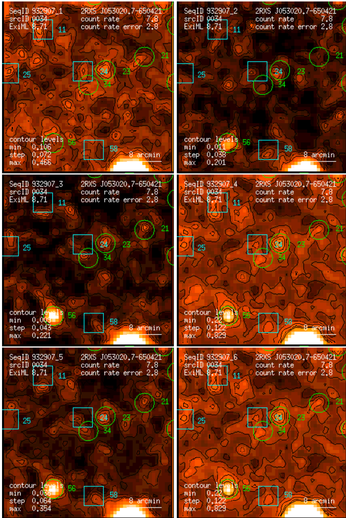
Figure 34: RASS 932907: detection 0034: band rate images, Gaussian filter: (1) PSPC channels 11 – 41, (2) 52 – 90, (3) 91 – 201, (4) 11 – 235, (5) 52 – 201, (6) 11 – 201. Broad band rates in counts/ks. Band rate contour levels in counts/ks/arcmin 2 .
