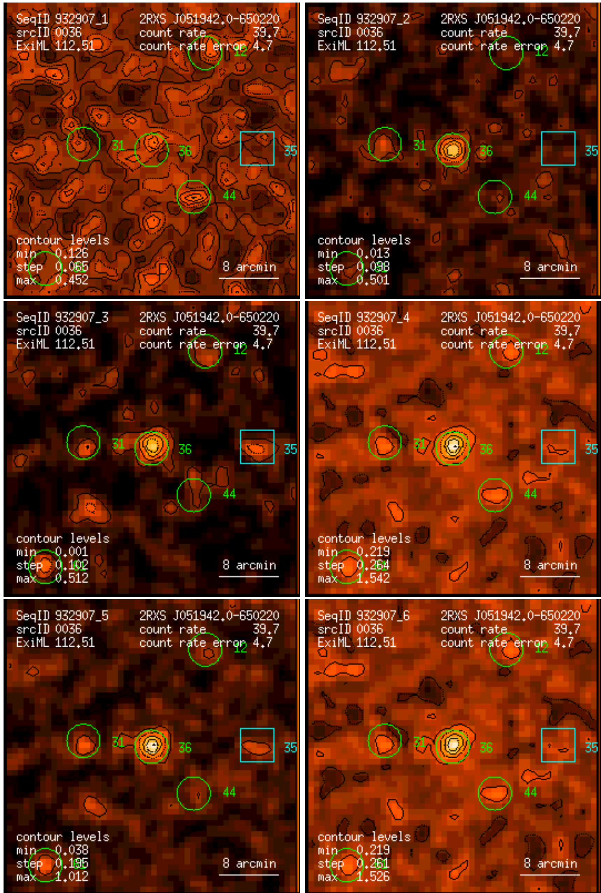
Figure 36: RASS 932907: detection 0036: band rate images, Gaussian filter: (1) PSPC channels 11 – 41, (2) 52 – 90, (3) 91 – 201, (4) 11 – 235, (5) 52 – 201, (6) 11 – 201. Broad band rates in counts/ks. Band rate contour levels in counts/ks/arcmin 2 .
