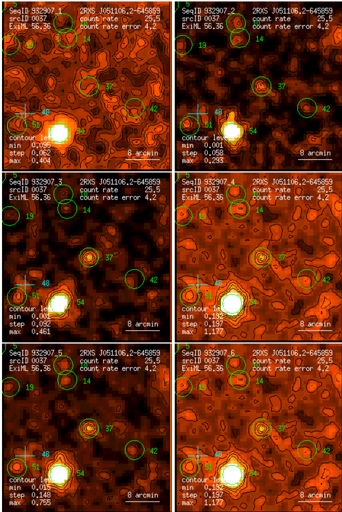
Figure 37: RASS 932907: detection 0037: band rate images, Gaussian filter: (1) PSPC channels 11 – 41, (2) 52 – 90, (3) 91 – 201, (4) 11 – 235, (5) 52 – 201, (6) 11 – 201. Broad band rates in counts/ks. Band rate contour levels in counts/ks/arcmin 2 .
