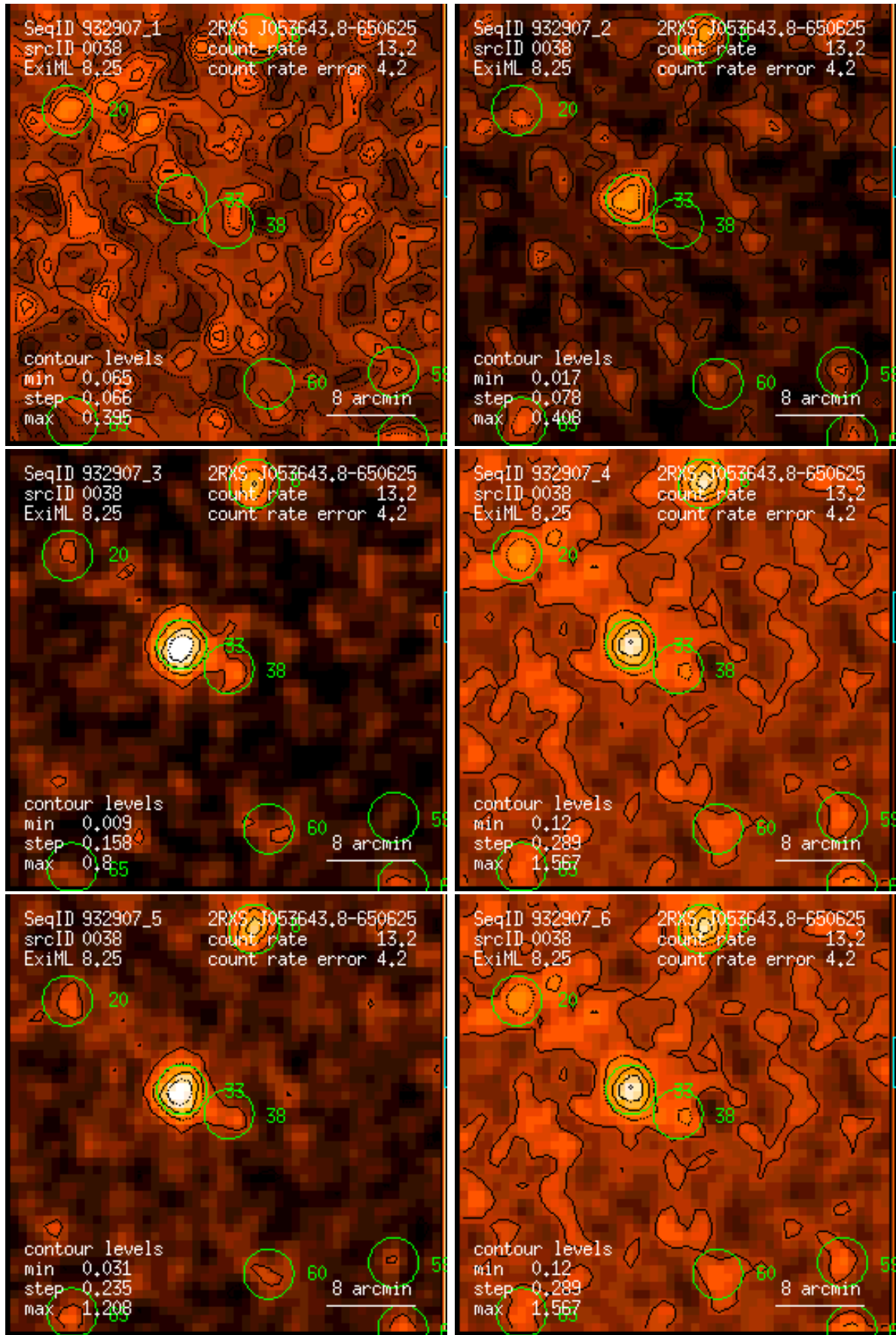
Figure 38: RASS 932907: detection 0038: band rate images, Gaussian filter: (1) PSPC channels 11 – 41, (2) 52 – 90, (3) 91 – 201, (4) 11 – 235, (5) 52 – 201, (6) 11 – 201. Broad band rates in counts/ks. Band rate contour levels in counts/ks/arcmin 2 .
