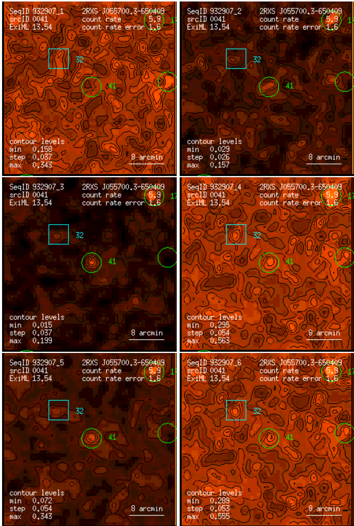
Figure 41: RASS 932907: detection 0041: band rate images, Gaussian filter: (1) PSPC channels 11 – 41, (2) 52 – 90, (3) 91 – 201, (4) 11 – 235, (5) 52 – 201, (6) 11 – 201. Broad band rates in counts/ks. Band rate contour levels in counts/ks/arcmin 2 .
