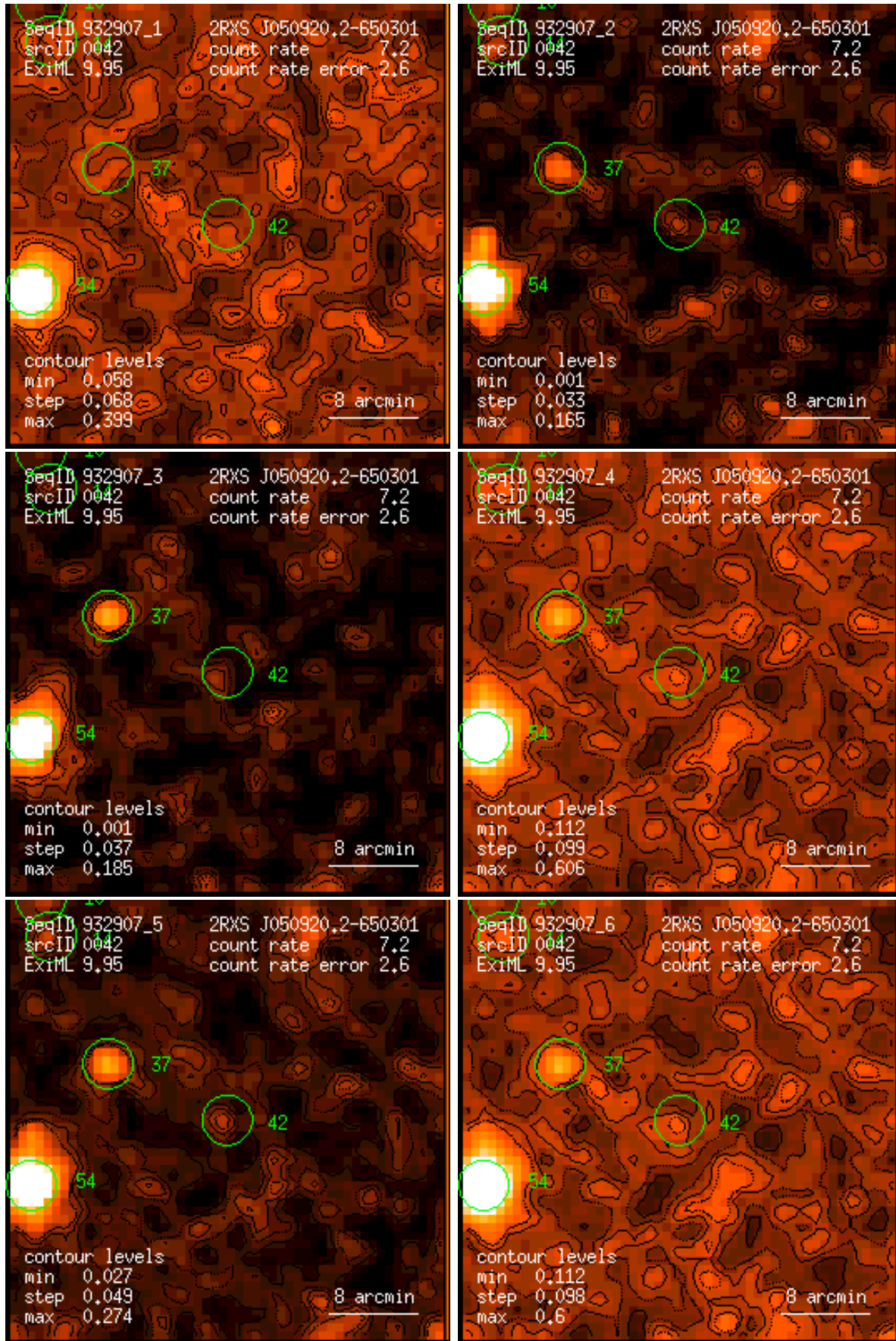
Figure 42: RASS 932907: detection 0042: band rate images, Gaussian filter: (1) PSPC channels 11 – 41, (2) 52 – 90, (3) 91 – 201, (4) 11 – 235, (5) 52 – 201, (6) 11 – 201. Broad band rates in counts/ks. Band rate contour levels in counts/ks/arcmin 2 .
