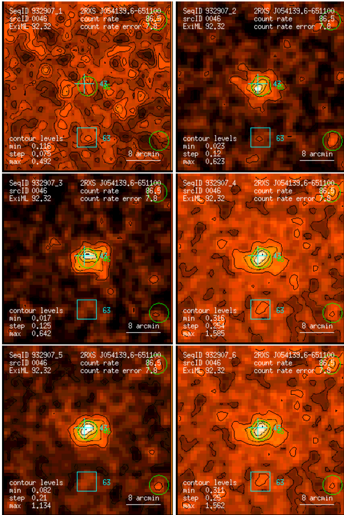
Figure 46: RASS 932907: detection 0046: band rate images, Gaussian filter: (1) PSPC channels 11 – 41, (2) 52 – 90, (3) 91 – 201, (4) 11 – 235, (5) 52 – 201, (6) 11 – 201. Broad band rates in counts/ks. Band rate contour levels in counts/ks/arcmin 2 .
