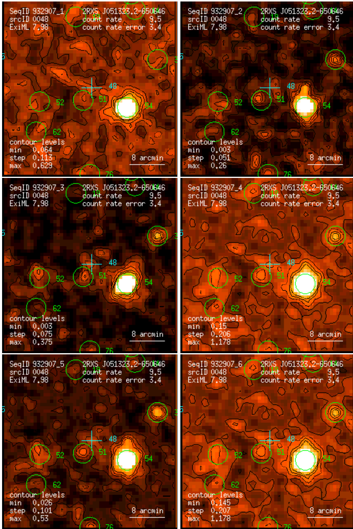
Figure 48: RASS 932907: detection 0048: band rate images, Gaussian filter: (1) PSPC channels 11 – 41, (2) 52 – 90, (3) 91 – 201, (4) 11 – 235, (5) 52 – 201, (6) 11 – 201. Broad band rates in counts/ks. Band rate contour levels in counts/ks/arcmin 2 .
