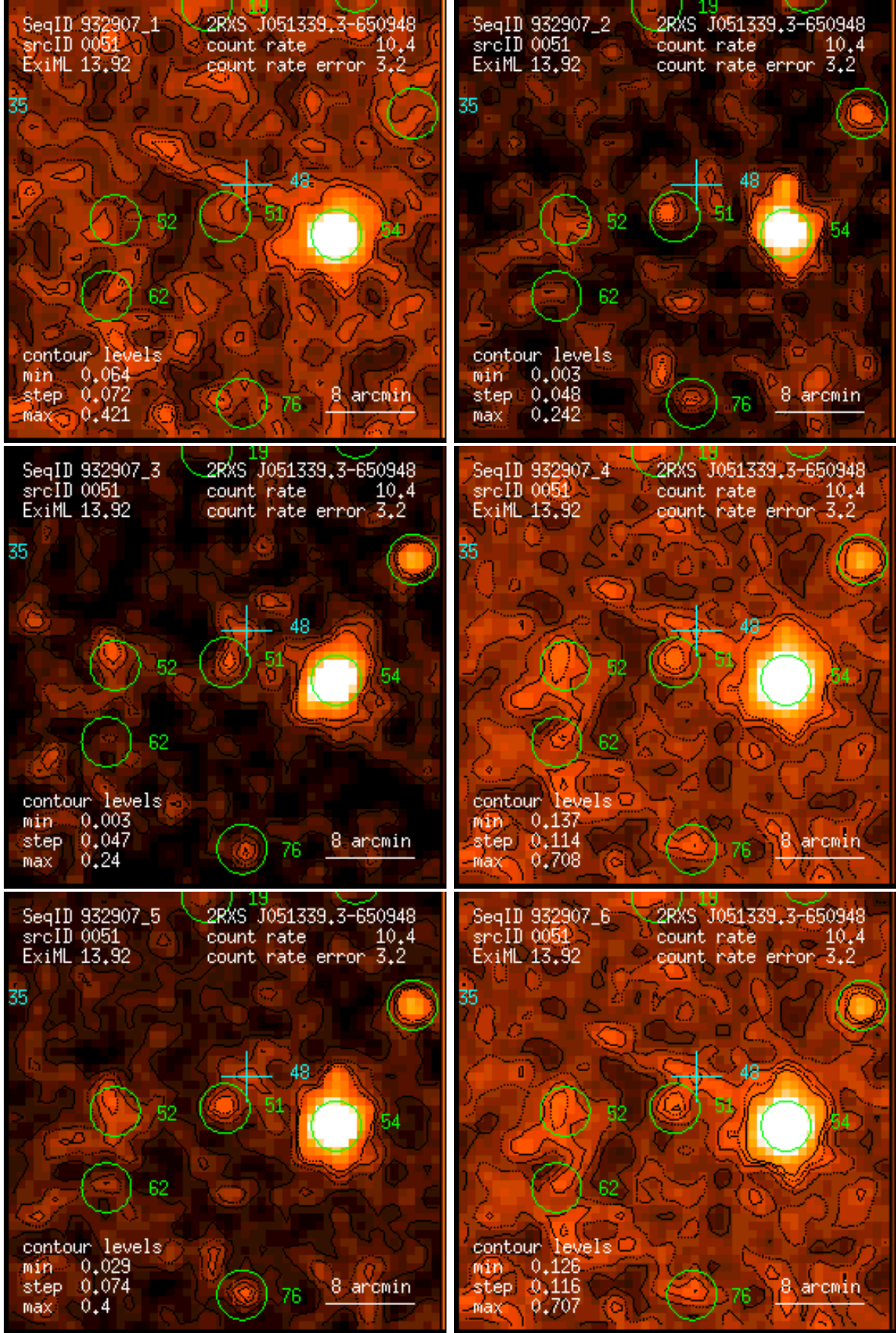
Figure 51: RASS 932907: detection 0051: band rate images, Gaussian filter: (1) PSPC channels 11 – 41, (2) 52 – 90, (3) 91 – 201, (4) 11 – 235, (5) 52 – 201, (6) 11 – 201. Broad band rates in counts/ks. Band rate contour levels in counts/ks/arcmin 2 .
