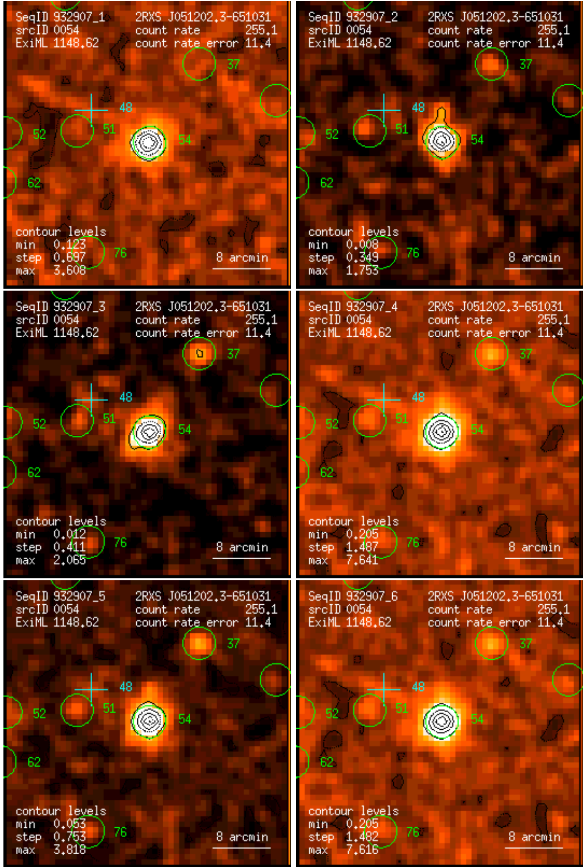
Figure 54: RASS 932907: detection 0054: band rate images, Gaussian filter: (1) PSPC channels 11 – 41, (2) 52 – 90, (3) 91 – 201, (4) 11 – 235, (5) 52 – 201, (6) 11 – 201. Broad band rates in counts/ks. Band rate contour levels in counts/ks/arcmin 2 .
