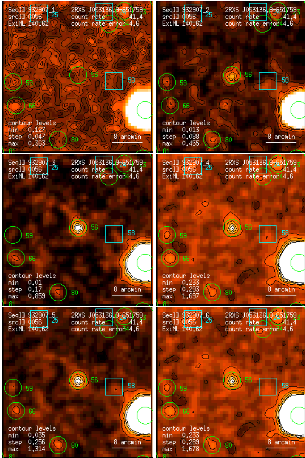
Figure 56: RASS 932907: detection 0056: band rate images, Gaussian filter: (1) PSPC channels 11 – 41, (2) 52 – 90, (3) 91 – 201, (4) 11 – 235, (5) 52 – 201, (6) 11 – 201. Broad band rates in counts/ks. Band rate contour levels in counts/ks/arcmin 2 .
