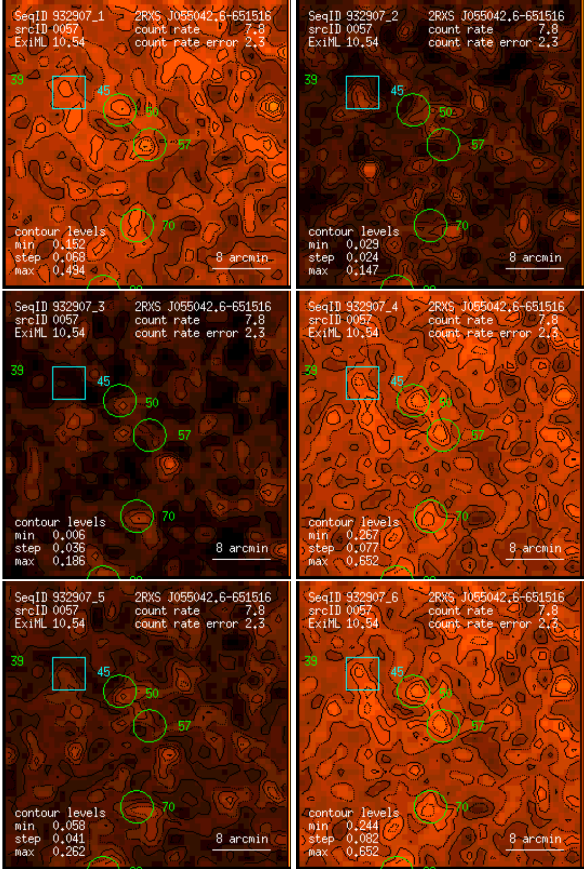
Figure 57: RASS 932907: detection 0057: band rate images, Gaussian filter: (1) PSPC channels 11 – 41, (2) 52 – 90, (3) 91 – 201, (4) 11 – 235, (5) 52 – 201, (6) 11 – 201. Broad band rates in counts/ks. Band rate contour levels in counts/ks/arcmin 2 .
