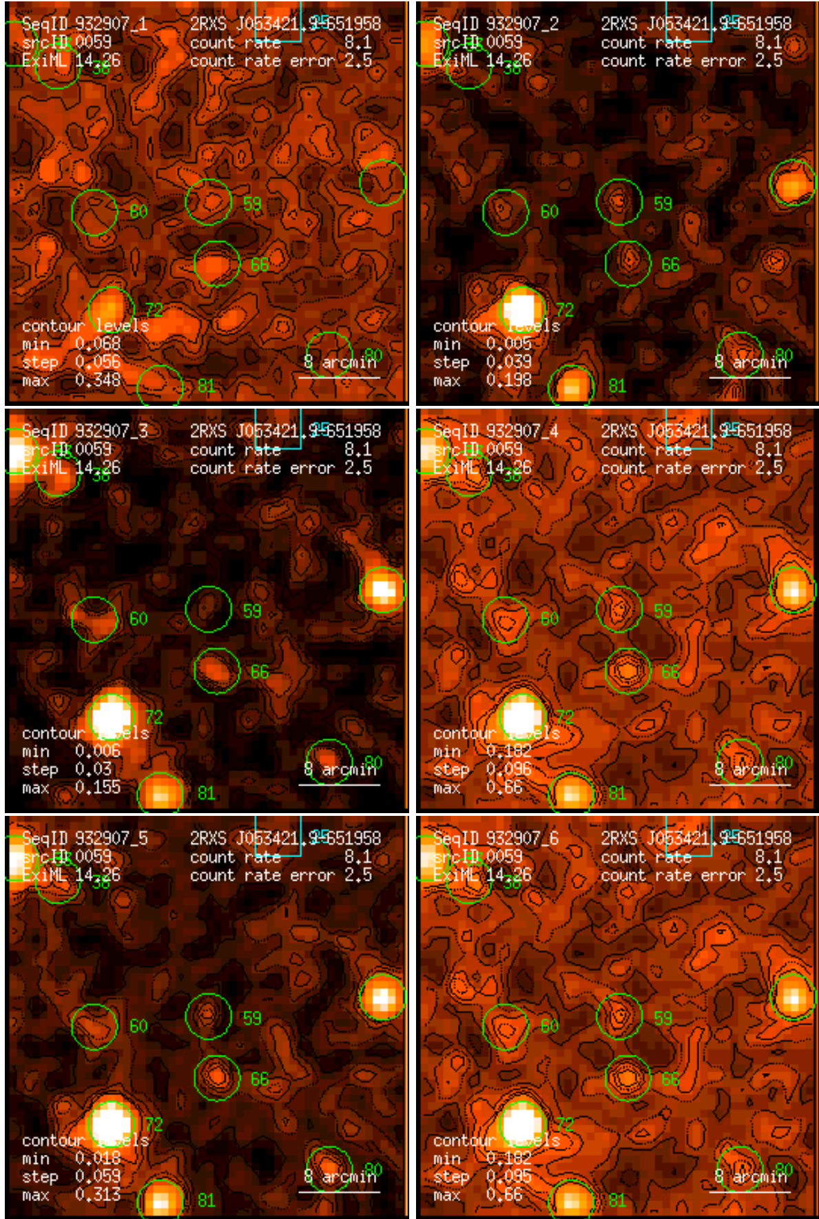
Figure 59: RASS 932907: detection 0059: band rate images, Gaussian filter: (1) PSPC channels 11 – 41, (2) 52 – 90, (3) 91 – 201, (4) 11 – 235, (5) 52 – 201, (6) 11 – 201. Broad band rates in counts/ks. Band rate contour levels in counts/ks/arcmin 2 .
