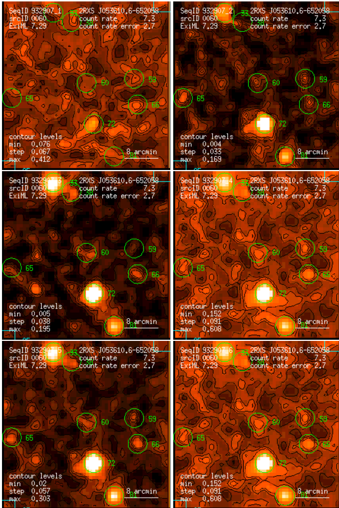
Figure 60: RASS 932907: detection 0060: band rate images, Gaussian filter: (1) PSPC channels 11 – 41, (2) 52 – 90, (3) 91 – 201, (4) 11 – 235, (5) 52 – 201, (6) 11 – 201. Broad band rates in counts/ks. Band rate contour levels in counts/ks/arcmin 2 .
