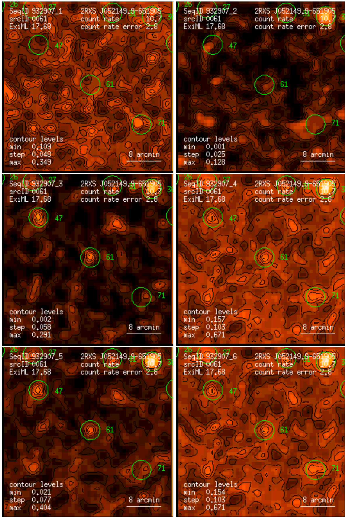
Figure 61: RASS 932907: detection 0061: band rate images, Gaussian filter: (1) PSPC channels 11 – 41, (2) 52 – 90, (3) 91 – 201, (4) 11 – 235, (5) 52 – 201, (6) 11 – 201. Broad band rates in counts/ks. Band rate contour levels in counts/ks/arcmin 2 .
