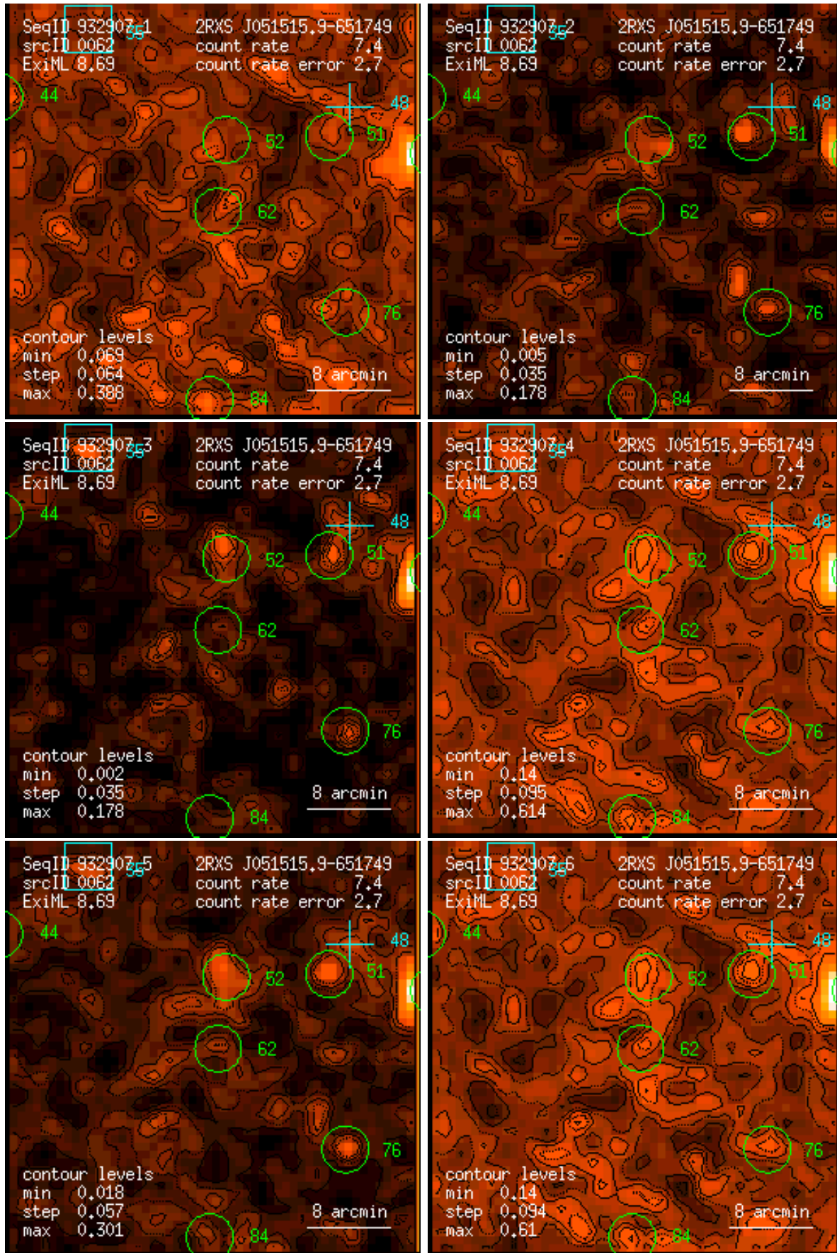
Figure 62: RASS 932907: detection 0062: band rate images, Gaussian filter: (1) PSPC channels 11 – 41, (2) 52 – 90, (3) 91 – 201, (4) 11 – 235, (5) 52 – 201, (6) 11 – 201. Broad band rates in counts/ks. Band rate contour levels in counts/ks/arcmin 2 .
