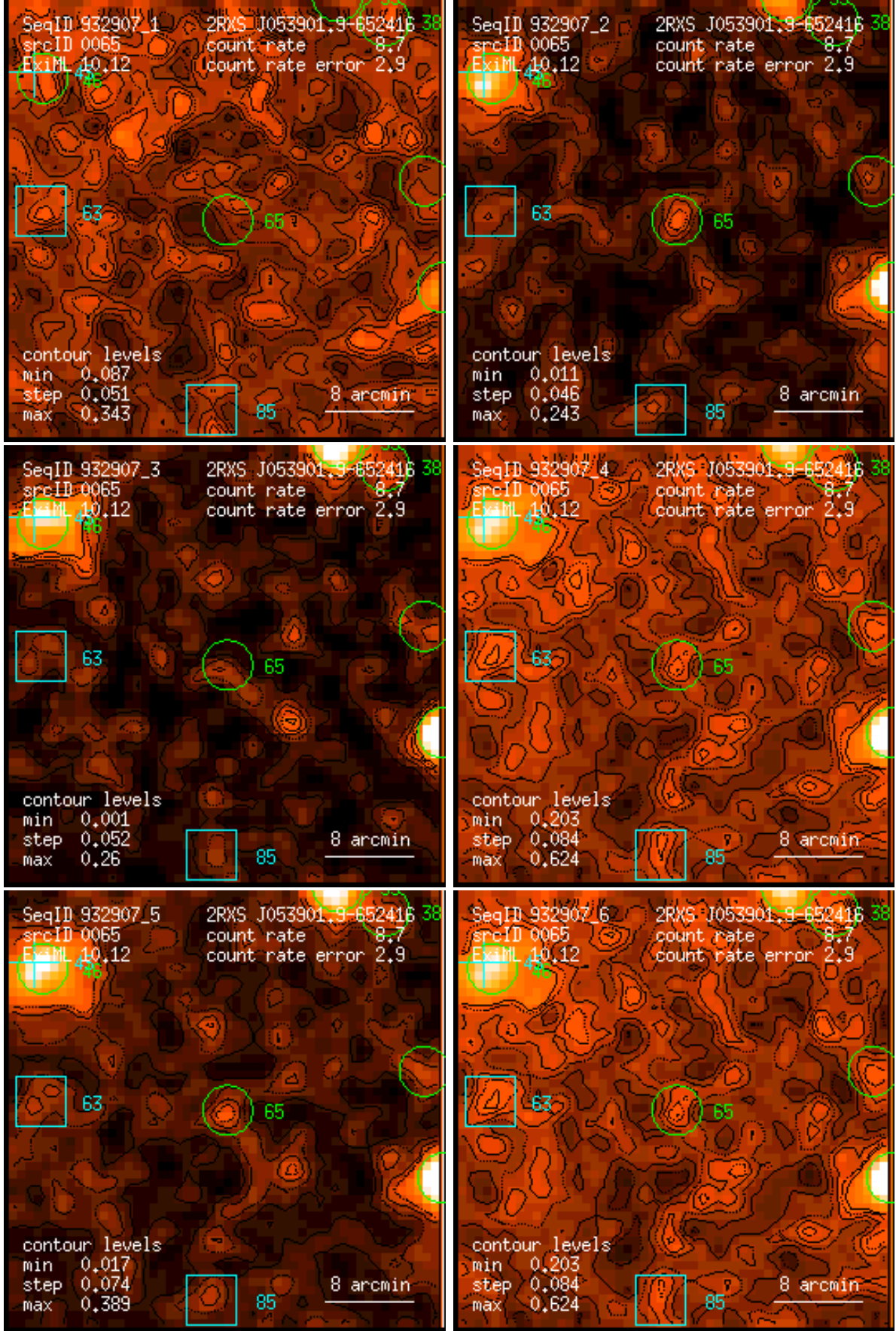
Figure 65: RASS 932907: detection 0065: band rate images, Gaussian filter: (1) PSPC channels 11 – 41, (2) 52 – 90, (3) 91 – 201, (4) 11 – 235, (5) 52 – 201, (6) 11 – 201. Broad band rates in counts/ks. Band rate contour levels in counts/ks/arcmin 2 .
