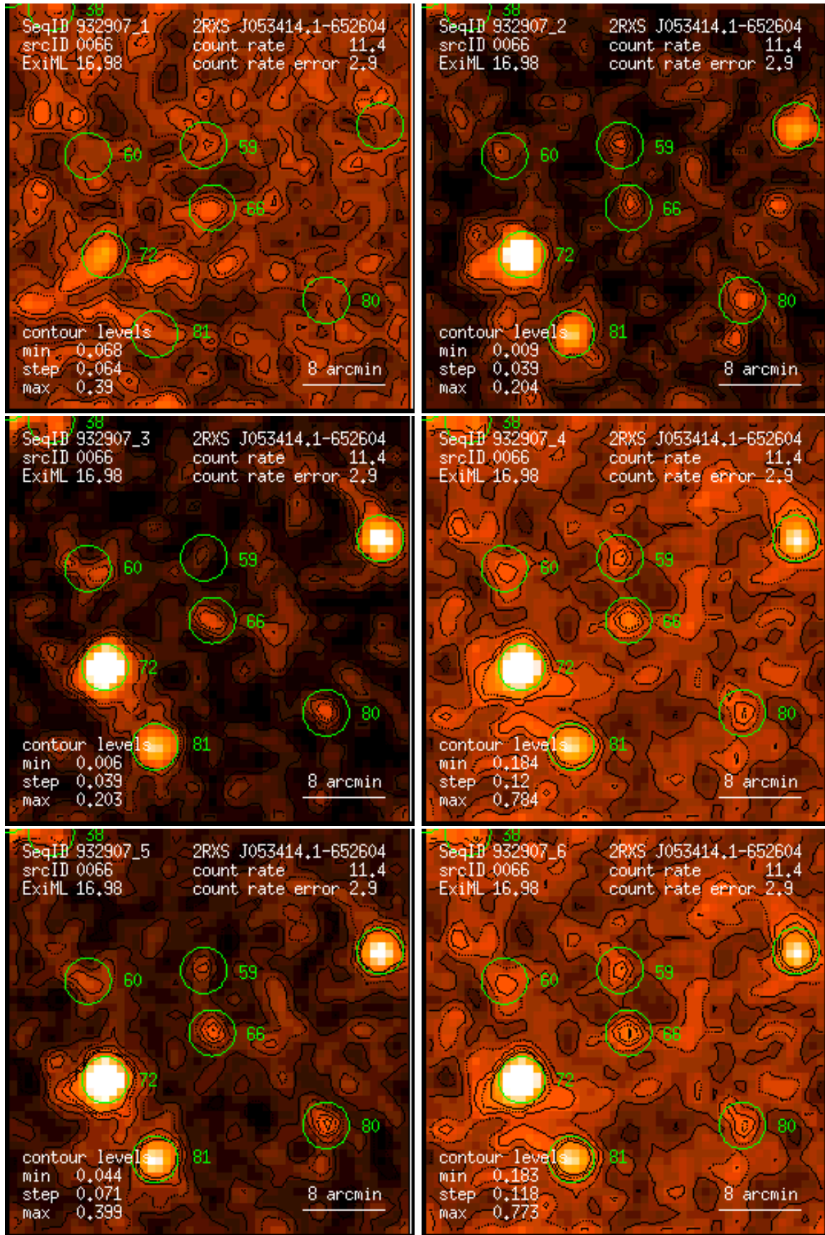
Figure 66: RASS 932907: detection 0066: band rate images, Gaussian filter: (1) PSPC channels 11 – 41, (2) 52 – 90, (3) 91 – 201, (4) 11 – 235, (5) 52 – 201, (6) 11 – 201. Broad band rates in counts/ks. Band rate contour levels in counts/ks/arcmin 2 .
