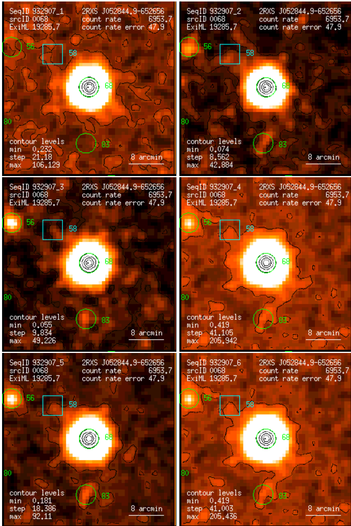
Figure 68: RASS 932907: detection 0068: band rate images, Gaussian filter: (1) PSPC channels 11 – 41, (2) 52 – 90, (3) 91 – 201, (4) 11 – 235, (5) 52 – 201, (6) 11 – 201. Broad band rates in counts/ks. Band rate contour levels in counts/ks/arcmin 2 .
