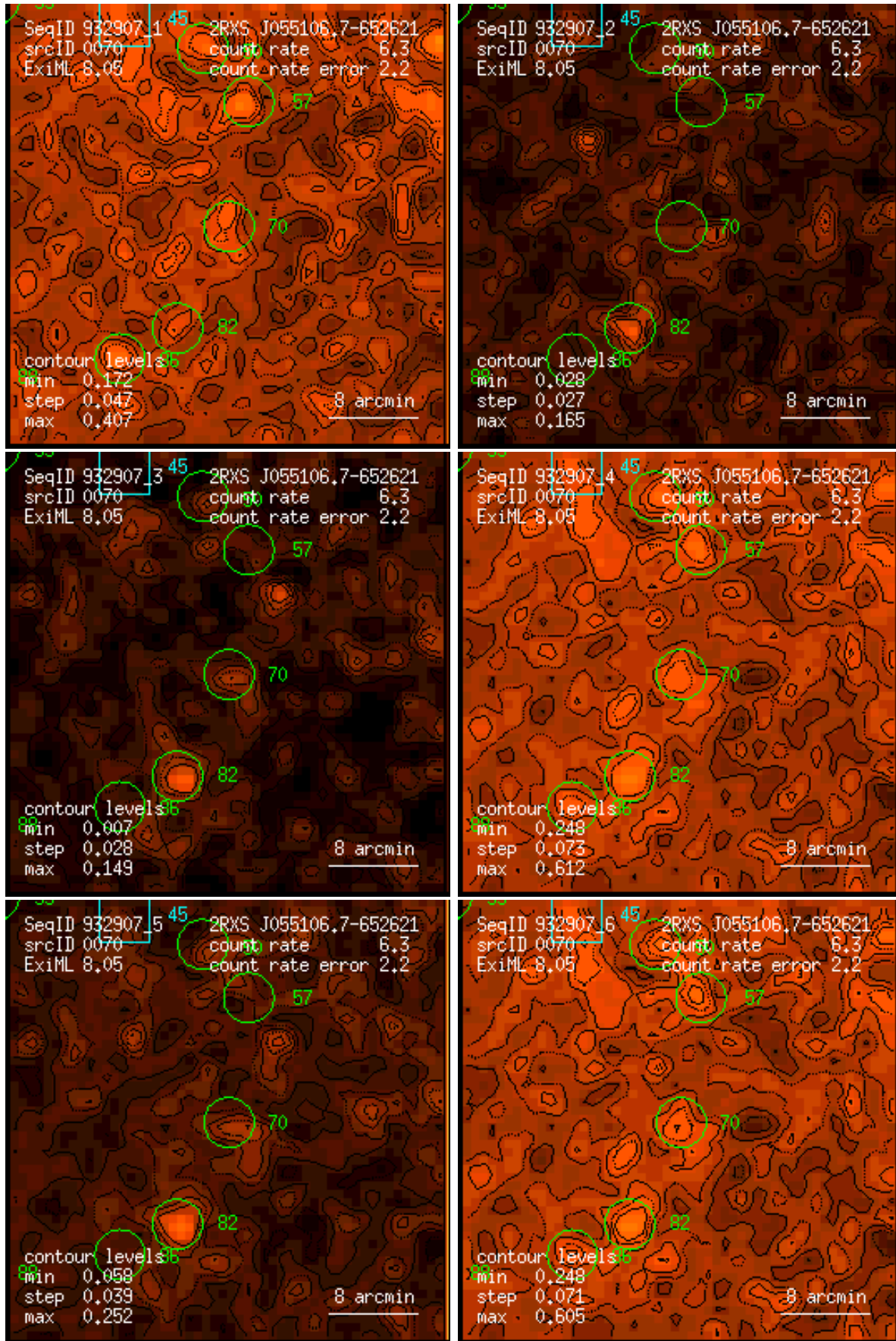
Figure 70: RASS 932907: detection 0070: band rate images, Gaussian filter: (1) PSPC channels 11 – 41, (2) 52 – 90, (3) 91 – 201, (4) 11 – 235, (5) 52 – 201, (6) 11 – 201. Broad band rates in counts/ks. Band rate contour levels in counts/ks/arcmin 2 .
