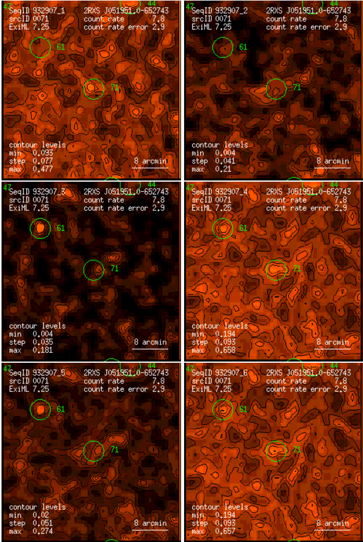
Figure 71: RASS 932907: detection 0071: band rate images, Gaussian filter: (1) PSPC channels 11 – 41, (2) 52 – 90, (3) 91 – 201, (4) 11 – 235, (5) 52 – 201, (6) 11 – 201. Broad band rates in counts/ks. Band rate contour levels in counts/ks/arcmin 2 .
