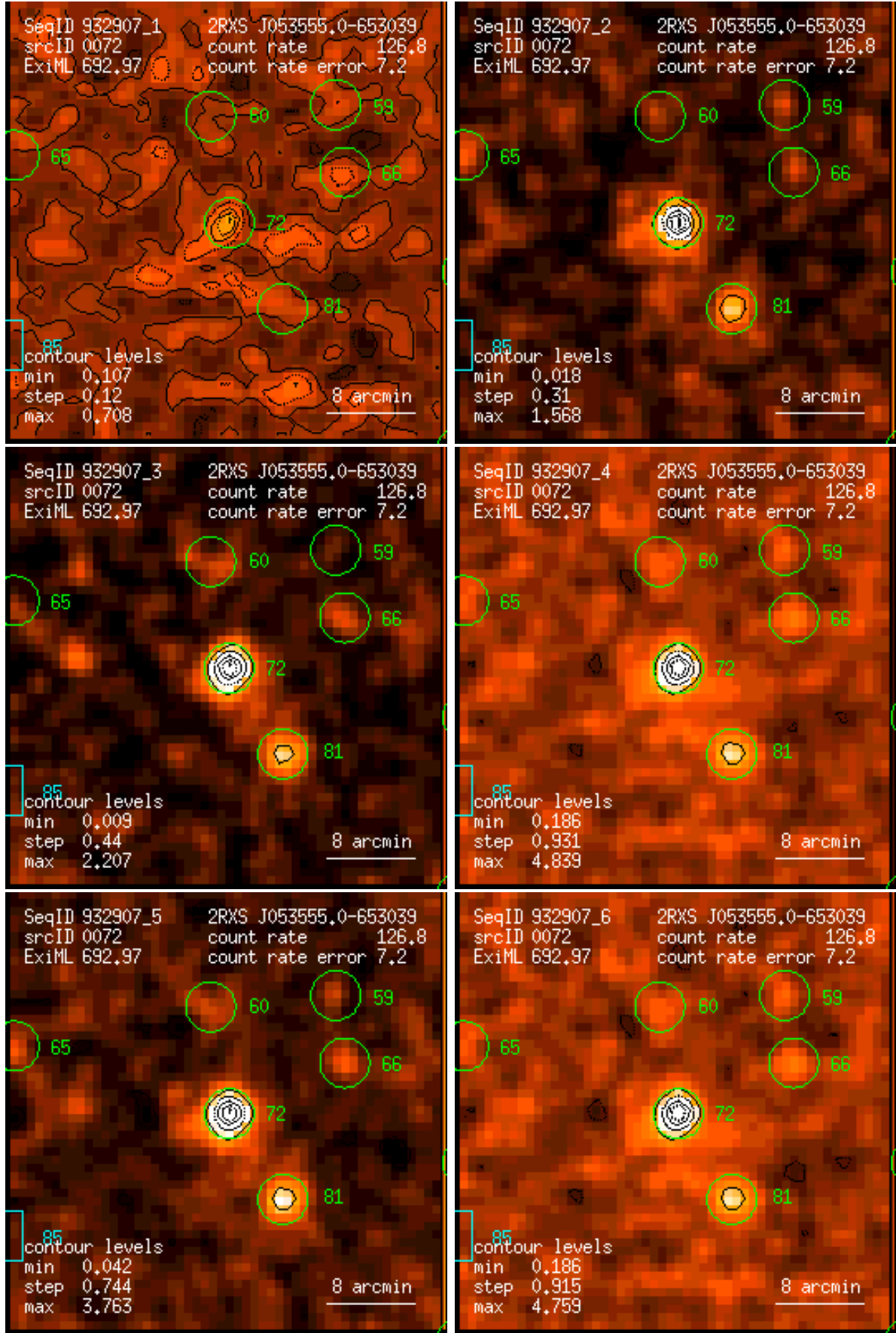
Figure 72: RASS 932907: detection 0072: band rate images, Gaussian filter: (1) PSPC channels 11 – 41, (2) 52 – 90, (3) 91 – 201, (4) 11 – 235, (5) 52 – 201, (6) 11 – 201. Broad band rates in counts/ks. Band rate contour levels in counts/ks/arcmin 2 .
