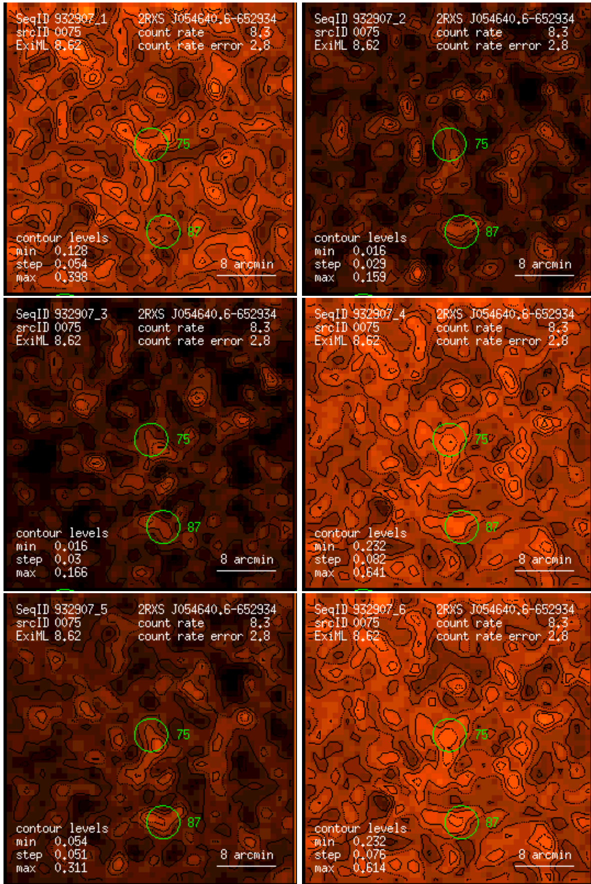
Figure 75: RASS 932907: detection 0075: band rate images, Gaussian filter: (1) PSPC channels 11 – 41, (2) 52 – 90, (3) 91 – 201, (4) 11 – 235, (5) 52 – 201, (6) 11 – 201. Broad band rates in counts/ks. Band rate contour levels in counts/ks/arcmin 2 .
