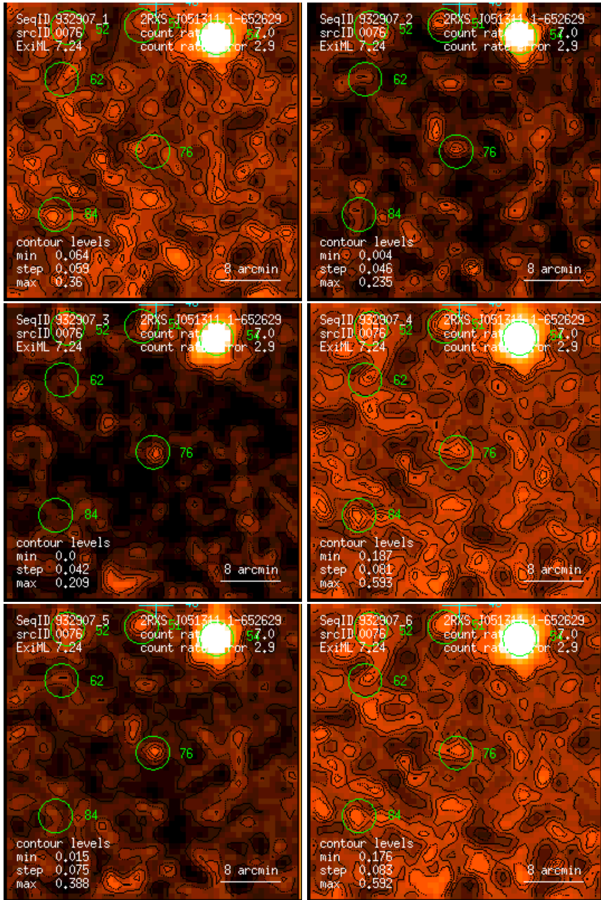
Figure 76: RASS 932907: detection 0076: band rate images, Gaussian filter: (1) PSPC channels 11 – 41, (2) 52 – 90, (3) 91 – 201, (4) 11 – 235, (5) 52 – 201, (6) 11 – 201. Broad band rates in counts/ks. Band rate contour levels in counts/ks/arcmin 2 .
