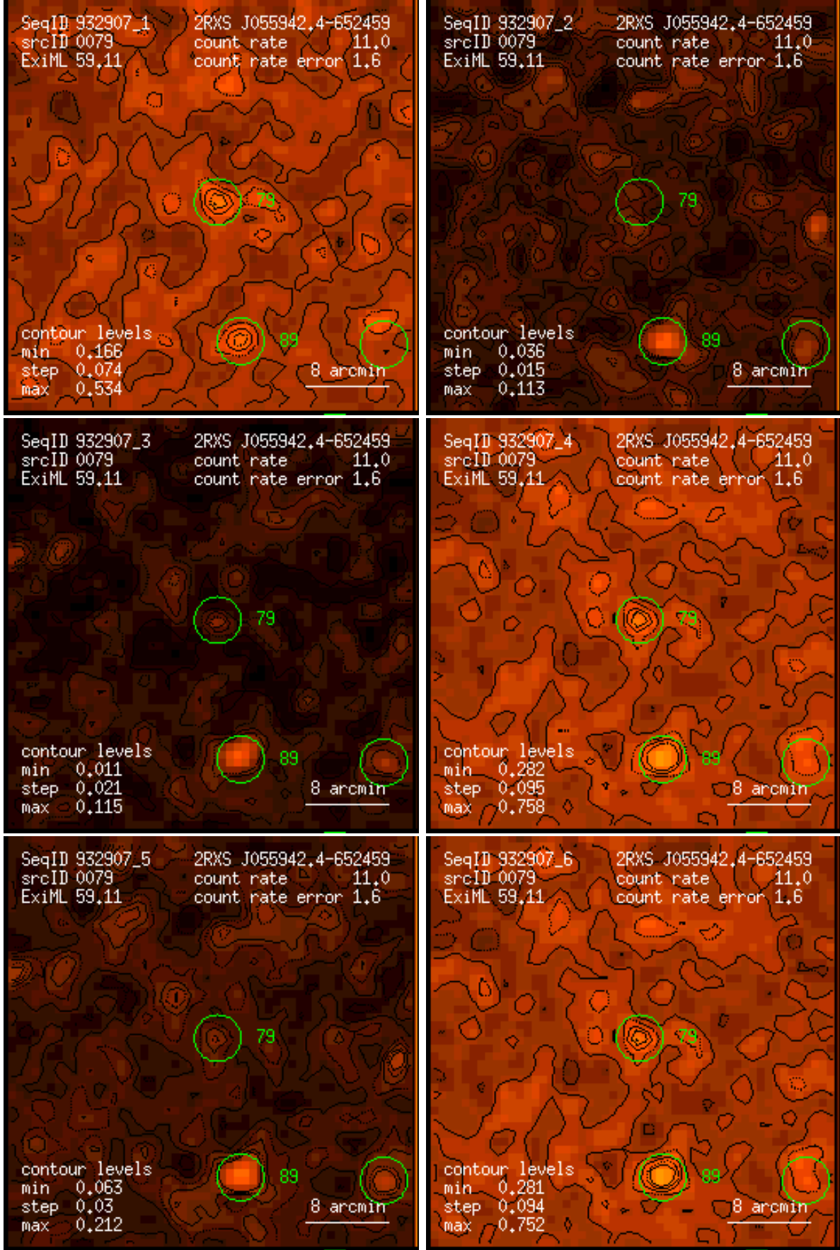
Figure 79: RASS 932907: detection 0079: band rate images, Gaussian filter: (1) PSPC channels 11 – 41, (2) 52 – 90, (3) 91 – 201, (4) 11 – 235, (5) 52 – 201, (6) 11 – 201. Broad band rates in counts/ks. Band rate contour levels in counts/ks/arcmin 2 .
