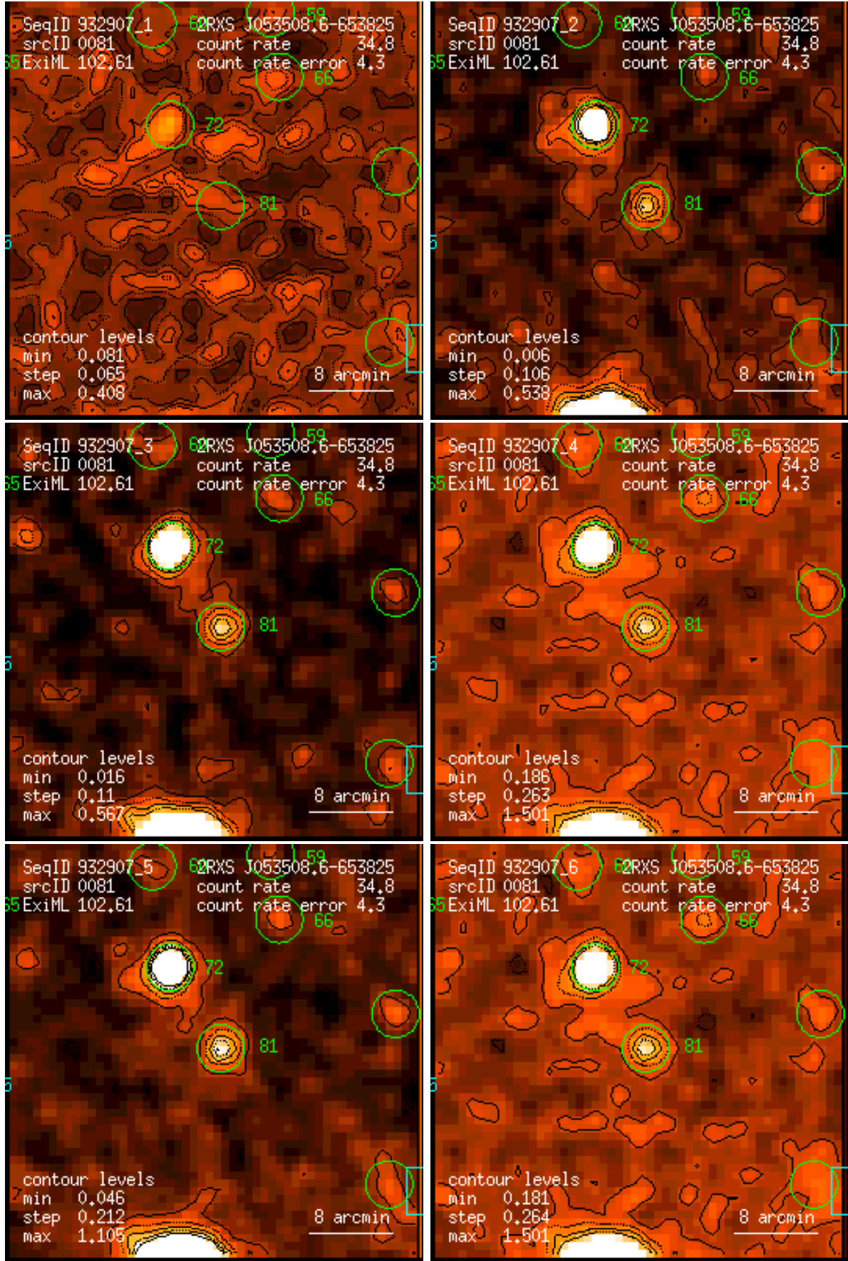
Figure 81: RASS 932907: detection 0081: band rate images, Gaussian filter: (1) PSPC channels 11 – 41, (2) 52 – 90, (3) 91 – 201, (4) 11 – 235, (5) 52 – 201, (6) 11 – 201. Broad band rates in counts/ks. Band rate contour levels in counts/ks/arcmin 2 .
