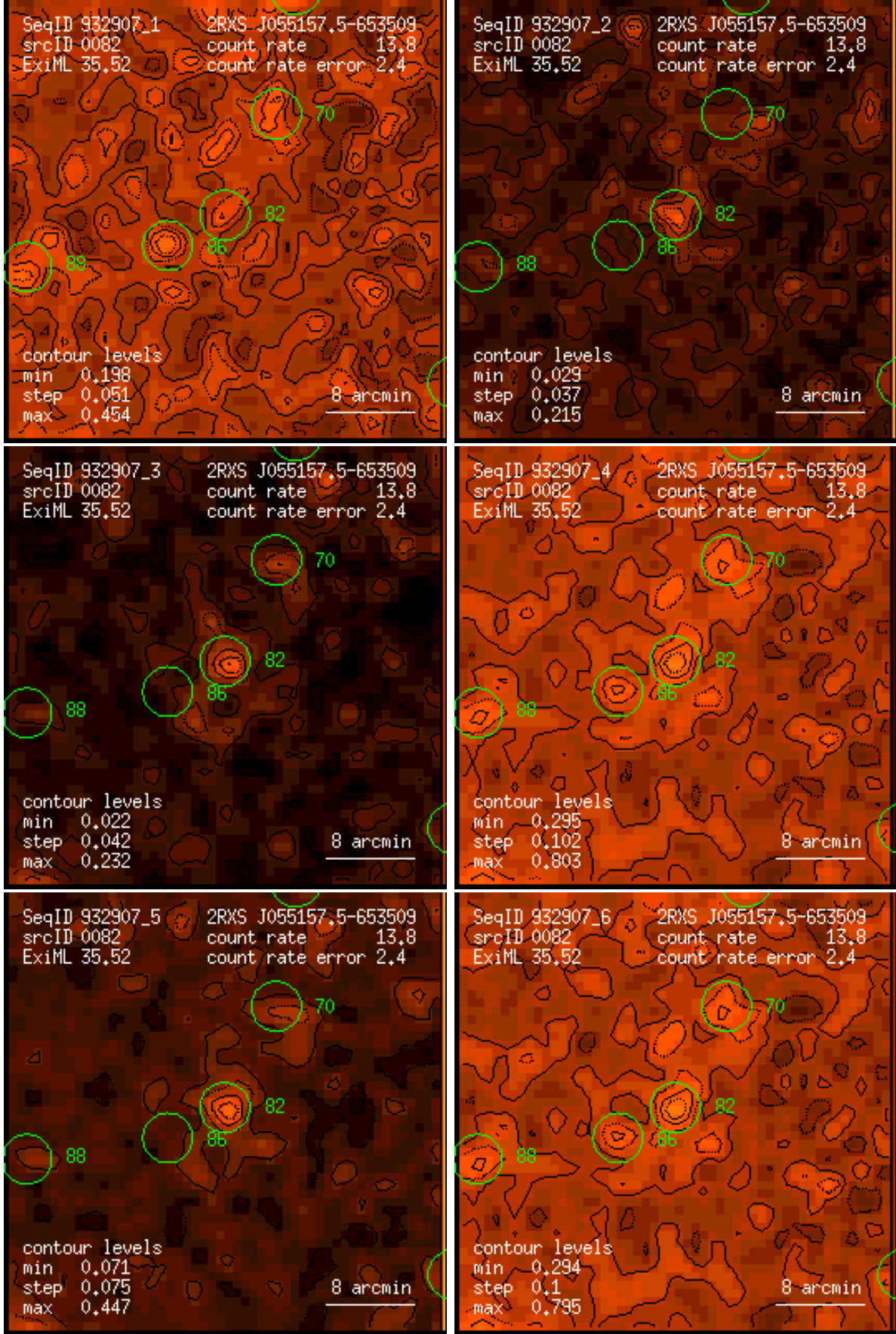
Figure 82: RASS 932907: detection 0082: band rate images, Gaussian filter: (1) PSPC channels 11 – 41, (2) 52 – 90, (3) 91 – 201, (4) 11 – 235, (5) 52 – 201, (6) 11 – 201. Broad band rates in counts/ks. Band rate contour levels in counts/ks/arcmin 2 .
