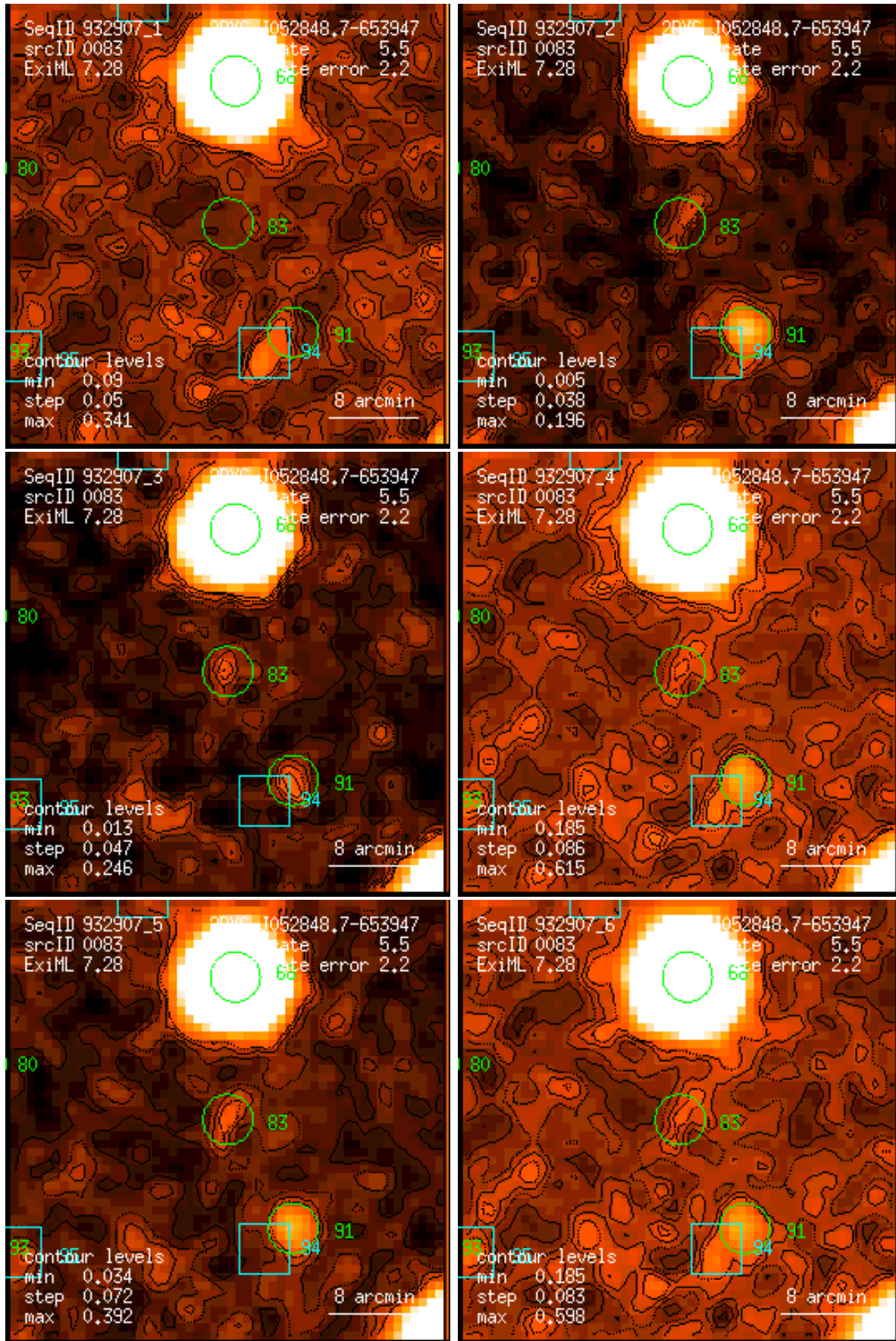
Figure 83: RASS 932907: detection 0083: band rate images, Gaussian filter: (1) PSPC channels 11 – 41, (2) 52 – 90, (3) 91 – 201, (4) 11 – 235, (5) 52 – 201, (6) 11 – 201. Broad band rates in counts/ks. Band rate contour levels in counts/ks/arcmin 2 .
