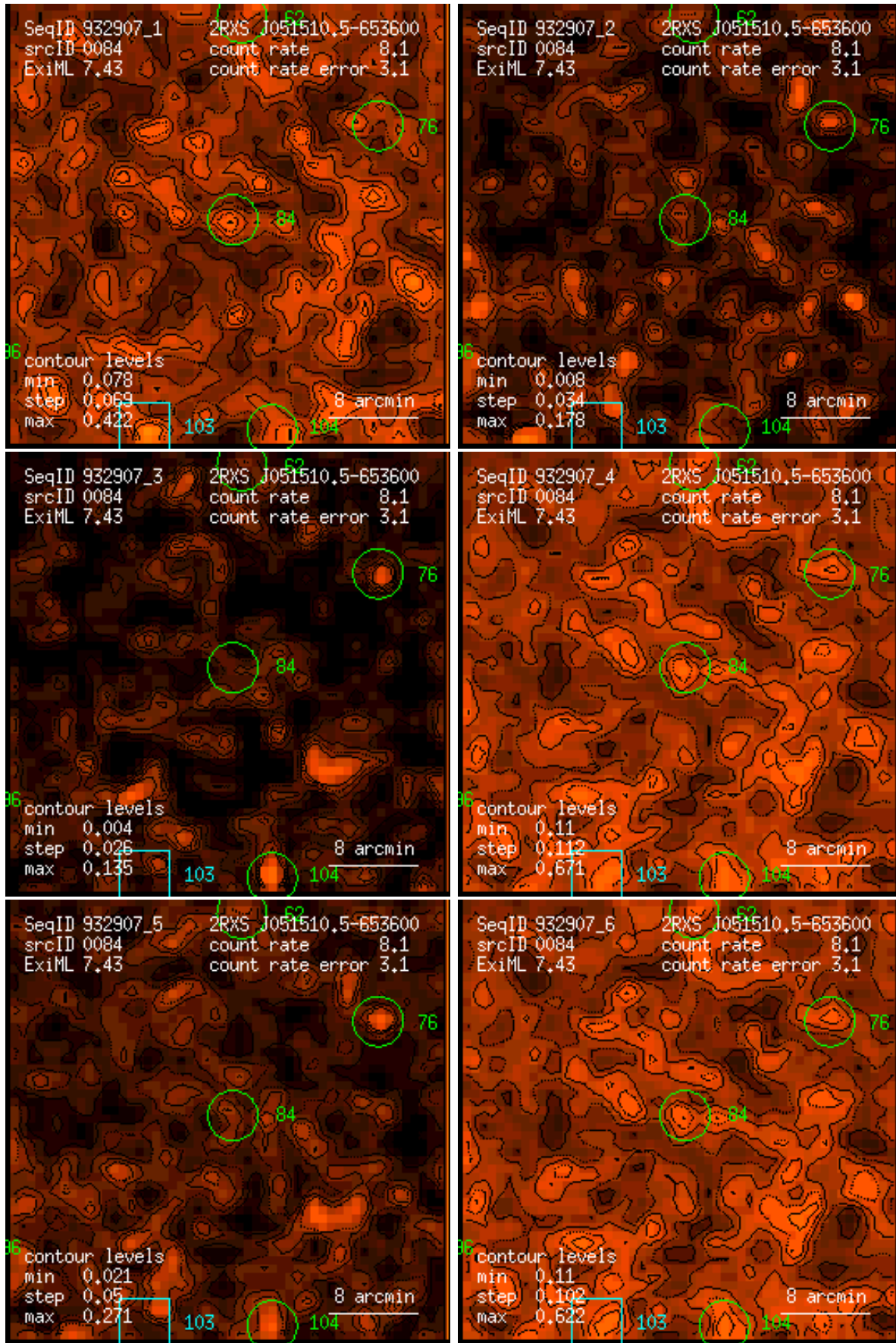
Figure 84: RASS 932907: detection 0084: band rate images, Gaussian filter: (1) PSPC channels 11 – 41, (2) 52 – 90, (3) 91 – 201, (4) 11 – 235, (5) 52 – 201, (6) 11 – 201. Broad band rates in counts/ks. Band rate contour levels in counts/ks/arcmin 2 .
