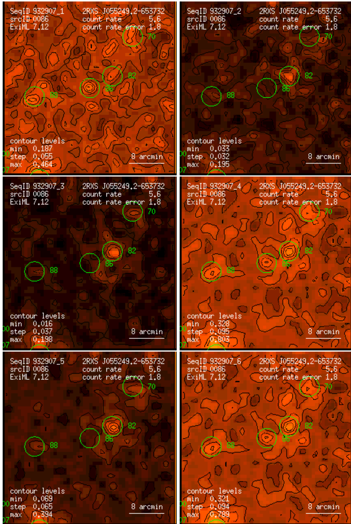
Figure 86: RASS 932907: detection 0086: band rate images, Gaussian filter: (1) PSPC channels 11 – 41, (2) 52 – 90, (3) 91 – 201, (4) 11 – 235, (5) 52 – 201, (6) 11 – 201. Broad band rates in counts/ks. Band rate contour levels in counts/ks/arcmin 2 .
